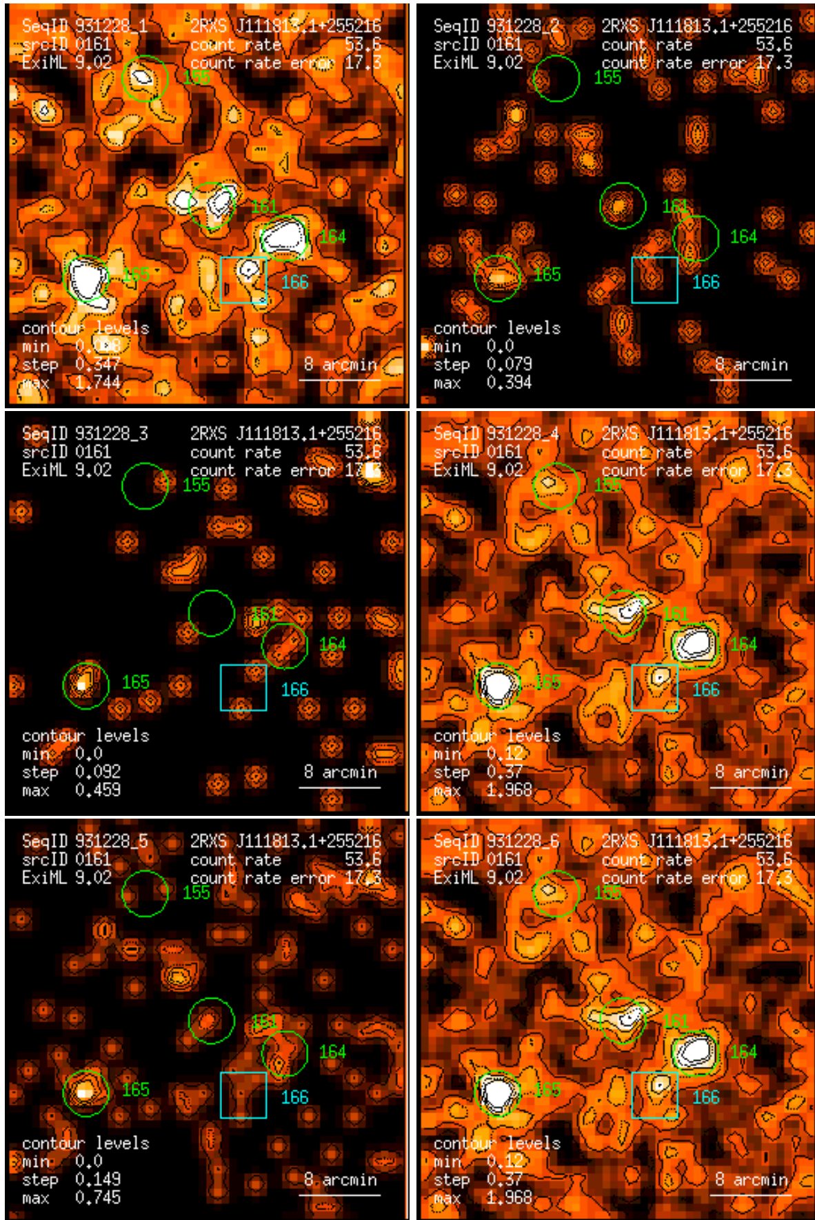
Figure 161: RASS 931228: detection 0161: band rate images, Gaussian filter: (1) PSPC channels 11 – 41, (2) 52 – 90, (3) 91 – 201, (4) 11 – 235, (5) 52 – 201, (6) 11 – 201. Broad band rates in counts/ks. Band rate contour levels in counts/ks/arcmin 2 .
