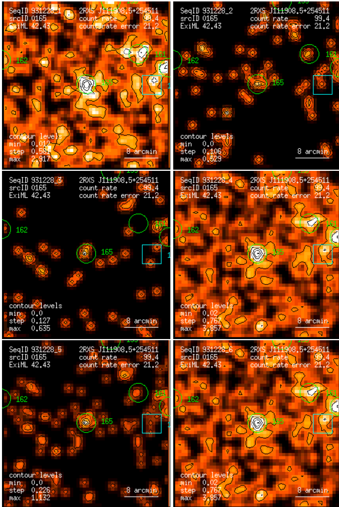
Figure 165: RASS 931228: detection 0165: band rate images, Gaussian filter: (1) PSPC channels 11 – 41, (2) 52 – 90, (3) 91 – 201, (4) 11 – 235, (5) 52 – 201, (6) 11 – 201. Broad band rates in counts/ks. Band rate contour levels in counts/ks/arcmin 2 .
