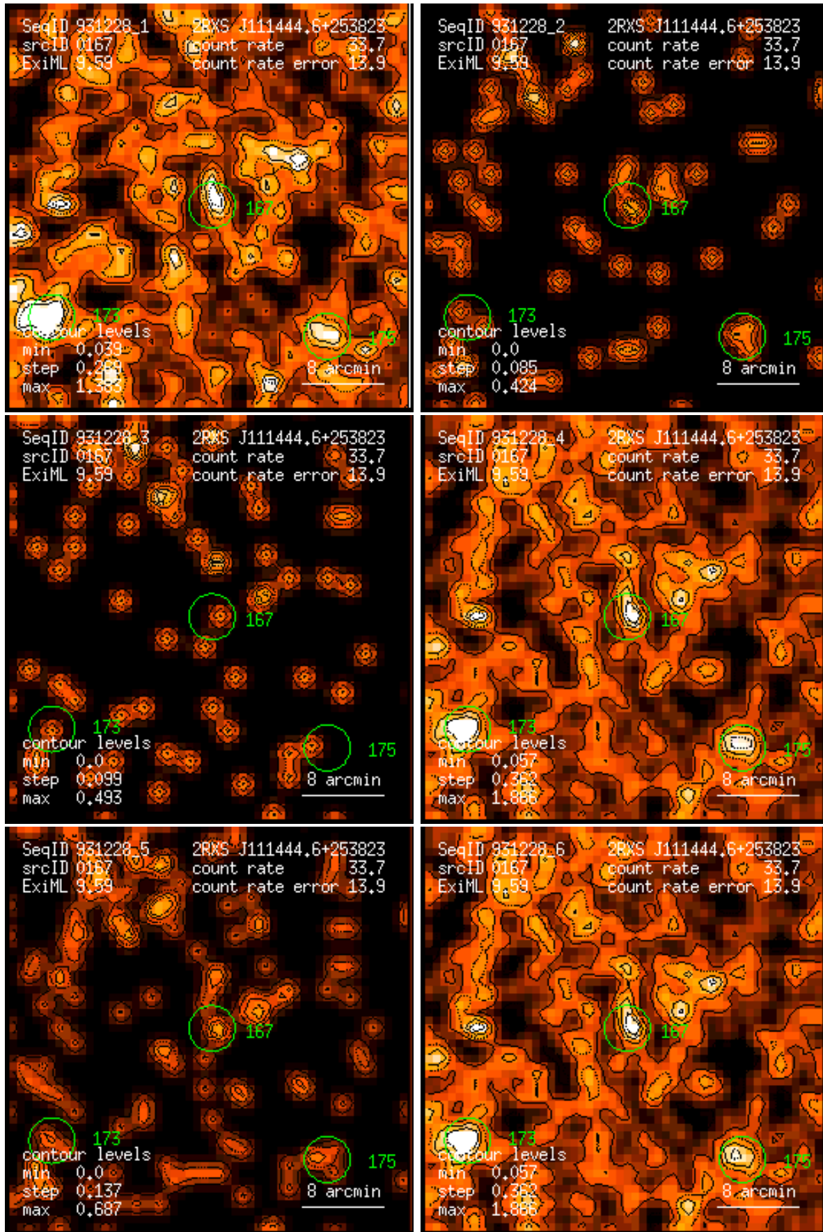
Figure 167: RASS 931228: detection 0167: band rate images, Gaussian filter: (1) PSPC channels 11 – 41, (2) 52 – 90, (3) 91 – 201, (4) 11 – 235, (5) 52 – 201, (6) 11 – 201. Broad band rates in counts/ks. Band rate contour levels in counts/ks/arcmin 2 .
