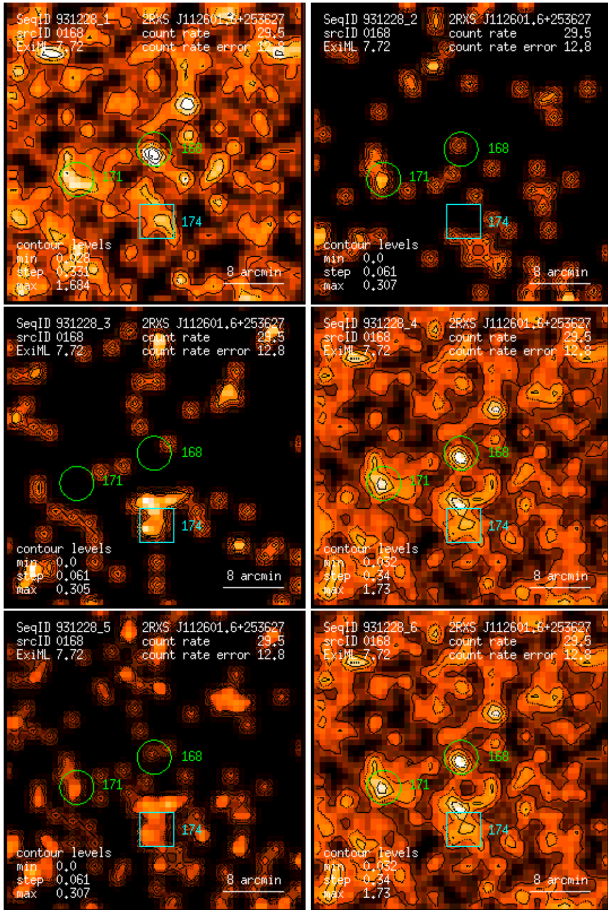
Figure 168: RASS 931228: detection 0168: band rate images, Gaussian filter: (1) PSPC channels 11 – 41, (2) 52 – 90, (3) 91 – 201, (4) 11 – 235, (5) 52 – 201, (6) 11 – 201. Broad band rates in counts/ks. Band rate contour levels in counts/ks/arcmin 2 .
