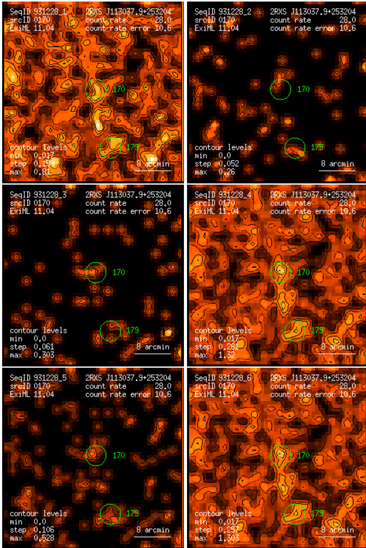
Figure 170: RASS 931228: detection 0170: band rate images, Gaussian filter: (1) PSPC channels 11 – 41, (2) 52 – 90, (3) 91 – 201, (4) 11 – 235, (5) 52 – 201, (6) 11 – 201. Broad band rates in counts/ks. Band rate contour levels in counts/ks/arcmin 2 .
