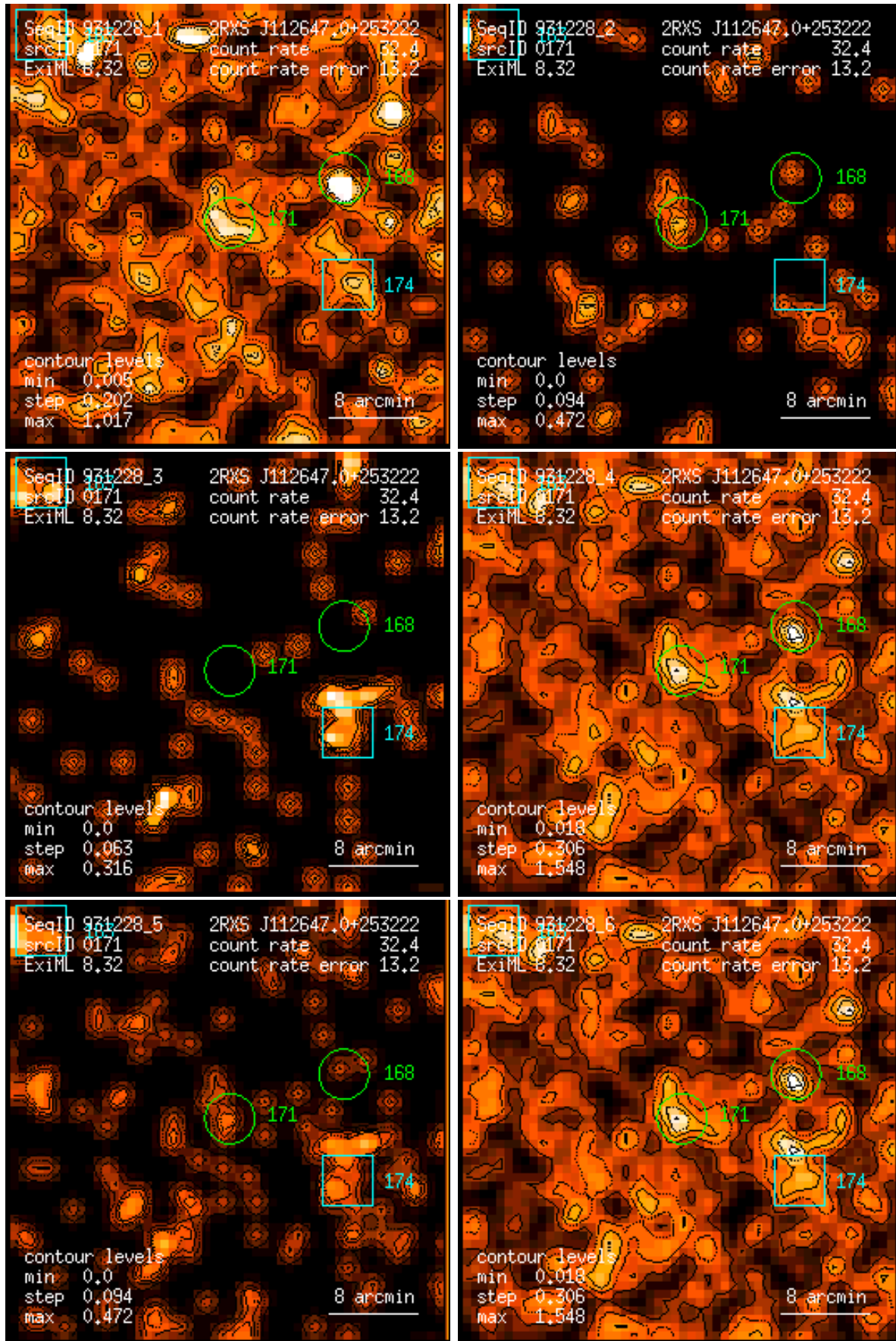
Figure 171: RASS 931228: detection 0171: band rate images, Gaussian filter: (1) PSPC channels 11 – 41, (2) 52 – 90, (3) 91 – 201, (4) 11 – 235, (5) 52 – 201, (6) 11 – 201. Broad band rates in counts/ks. Band rate contour levels in counts/ks/arcmin 2 .
