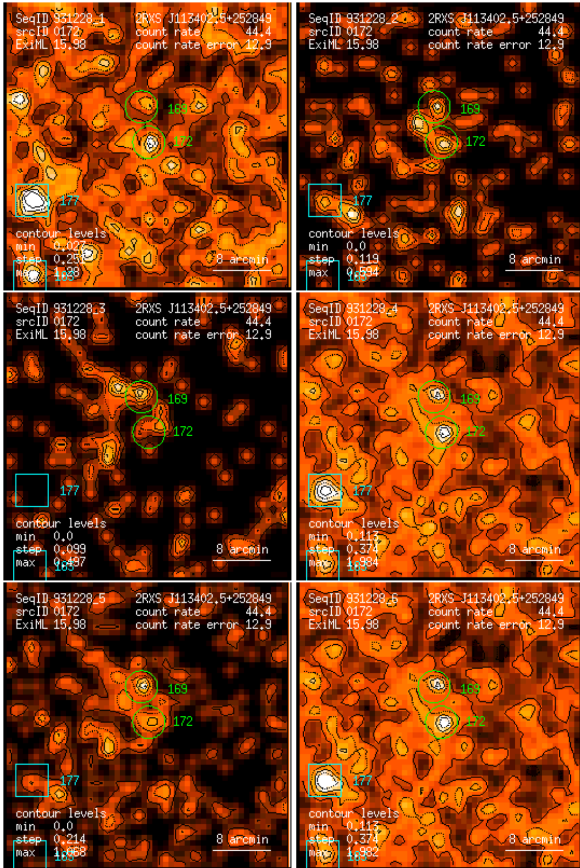
Figure 172: RASS 931228: detection 0172: band rate images, Gaussian filter: (1) PSPC channels 11 – 41, (2) 52 – 90, (3) 91 – 201, (4) 11 – 235, (5) 52 – 201, (6) 11 – 201. Broad band rates in counts/ks. Band rate contour levels in counts/ks/arcmin 2 .
