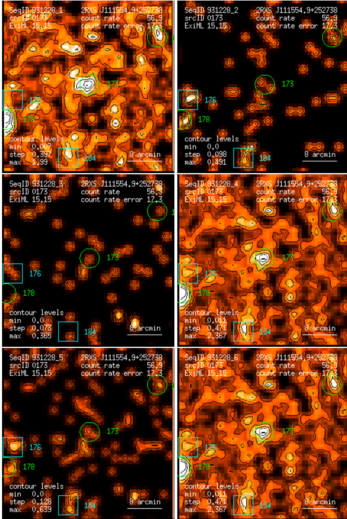
Figure 173: RASS 931228: detection 0173: band rate images, Gaussian filter: (1) PSPC channels 11 – 41, (2) 52 – 90, (3) 91 – 201, (4) 11 – 235, (5) 52 – 201, (6) 11 – 201. Broad band rates in counts/ks. Band rate contour levels in counts/ks/arcmin 2 .
