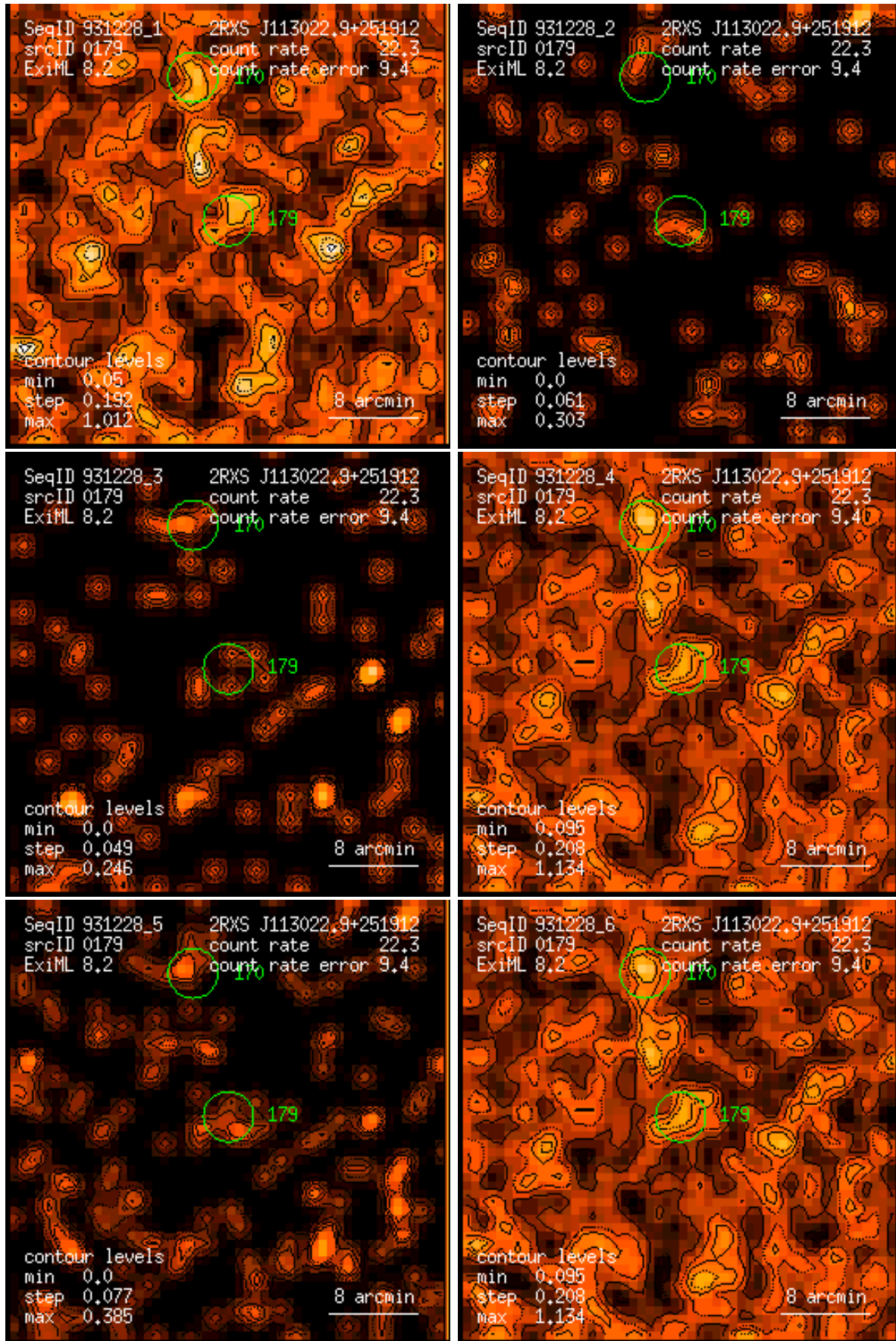
Figure 179: RASS 931228: detection 0179: band rate images, Gaussian filter: (1) PSPC channels 11 – 41, (2) 52 – 90, (3) 91 – 201, (4) 11 – 235, (5) 52 – 201, (6) 11 – 201. Broad band rates in counts/ks. Band rate contour levels in counts/ks/arcmin 2 .
