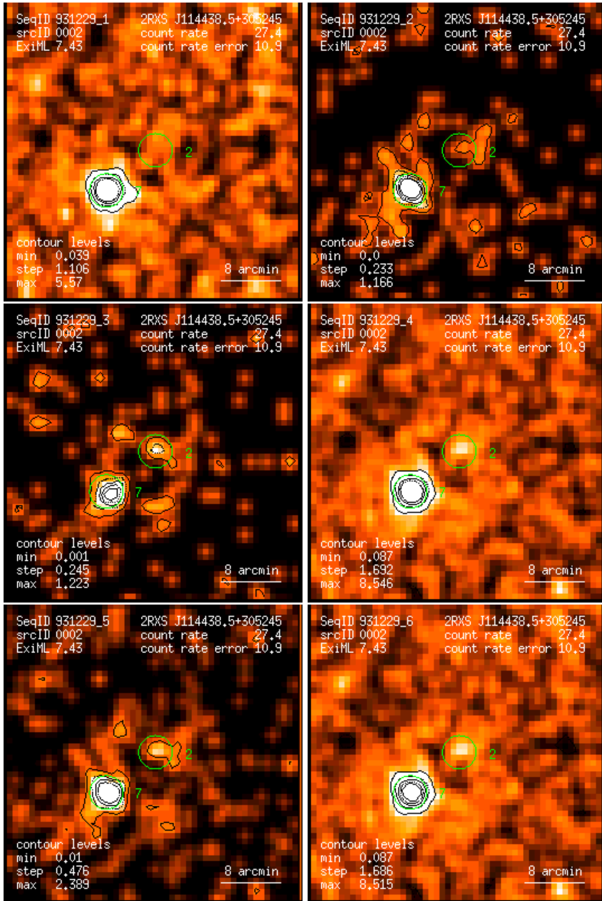
Figure 2: RASS 931229: detection 0002: band rate images, Gaussian filter: (1) PSPC channels 11 – 41, (2) 52 – 90, (3) 91 – 201, (4) 11 – 235, (5) 52 – 201, (6) 11 – 201. Broad band rates in counts/ks. Band rate contour levels in counts/ks/arcmin 2 .
