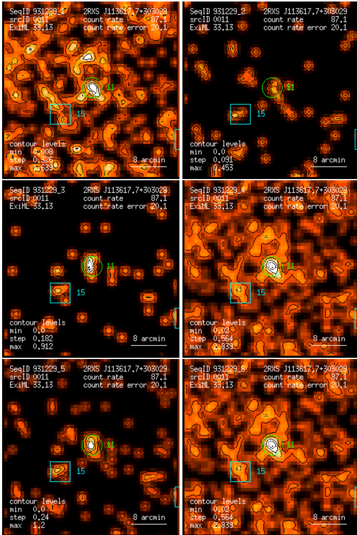
Figure 11: RASS 931229: detection 0011: band rate images, Gaussian filter: (1) PSPC channels 11 – 41, (2) 52 – 90, (3) 91 – 201, (4) 11 – 235, (5) 52 – 201, (6) 11 – 201. Broad band rates in counts/ks. Band rate contour levels in counts/ks/arcmin 2 .
