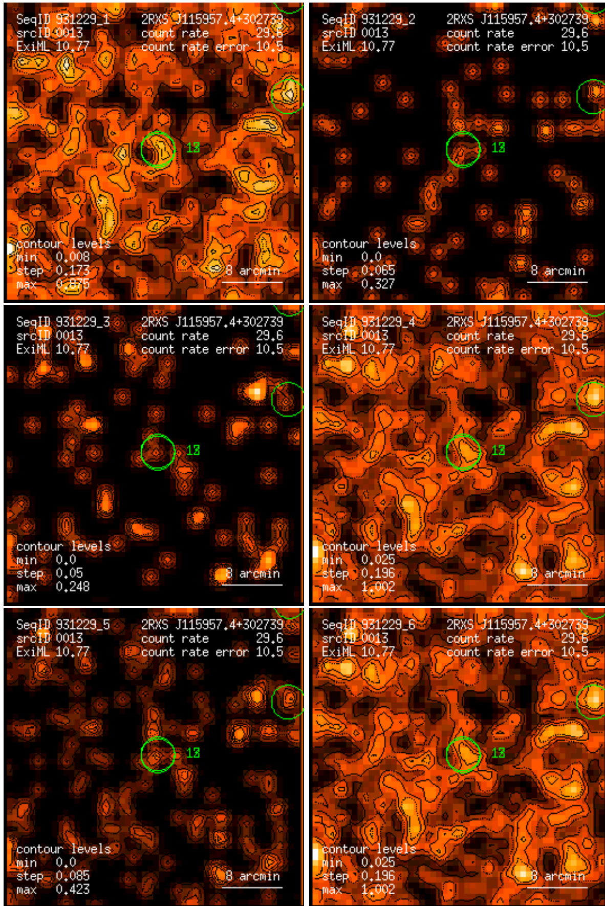
Figure 13: RASS 931229: detection 0013: band rate images, Gaussian filter: (1) PSPC channels 11 – 41, (2) 52 – 90, (3) 91 – 201, (4) 11 – 235, (5) 52 – 201, (6) 11 – 201. Broad band rates in counts/ks. Band rate contour levels in counts/ks/arcmin 2 .
