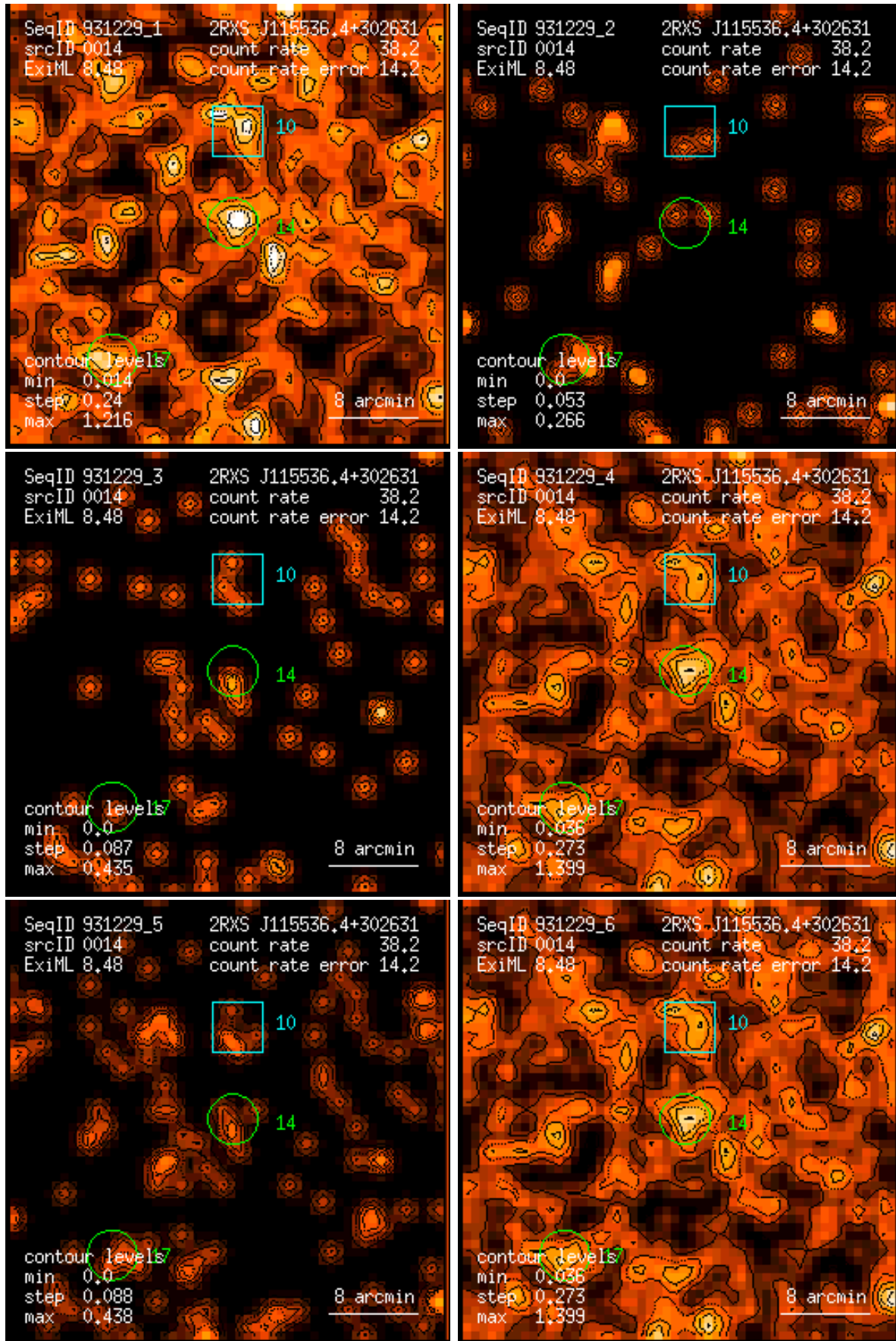
Figure 14: RASS 931229: detection 0014: band rate images, Gaussian filter: (1) PSPC channels 11 – 41, (2) 52 – 90, (3) 91 – 201, (4) 11 – 235, (5) 52 – 201, (6) 11 – 201. Broad band rates in counts/ks. Band rate contour levels in counts/ks/arcmin 2 .
