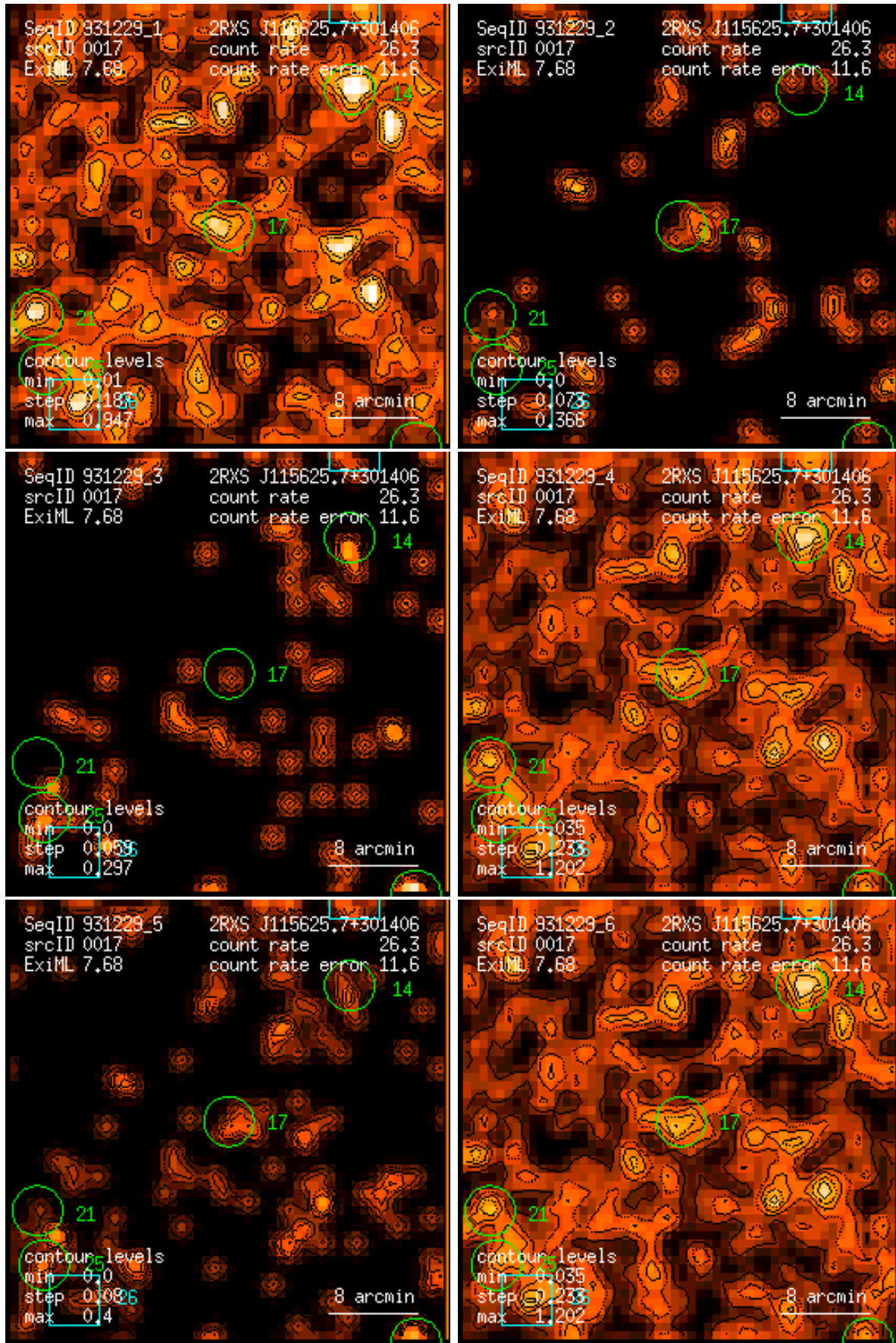
Figure 17: RASS 931229: detection 0017: band rate images, Gaussian filter: (1) PSPC channels 11 – 41, (2) 52 – 90, (3) 91 – 201, (4) 11 – 235, (5) 52 – 201, (6) 11 – 201. Broad band rates in counts/ks. Band rate contour levels in counts/ks/arcmin 2 .
