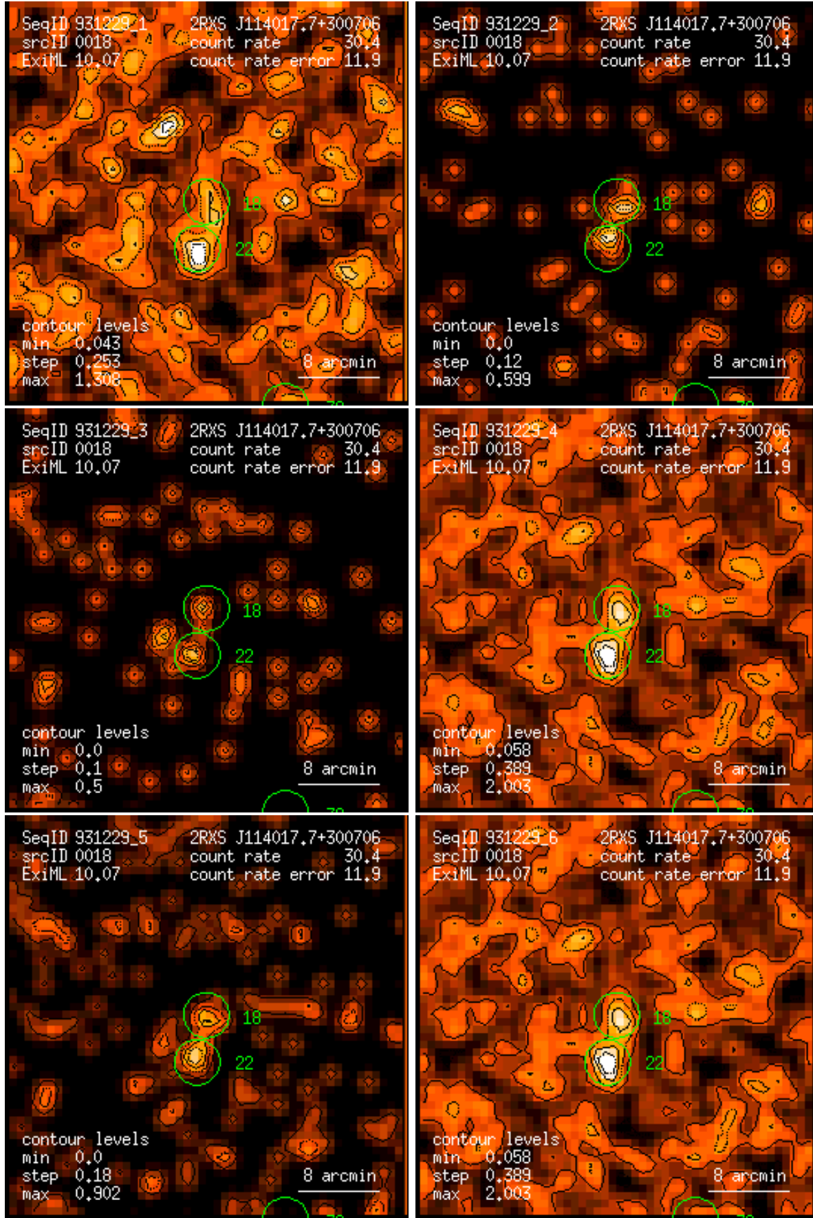
Figure 18: RASS 931229: detection 0018: band rate images, Gaussian filter: (1) PSPC channels 11 – 41, (2) 52 – 90, (3) 91 – 201, (4) 11 – 235, (5) 52 – 201, (6) 11 – 201. Broad band rates in counts/ks. Band rate contour levels in counts/ks/arcmin 2 .
