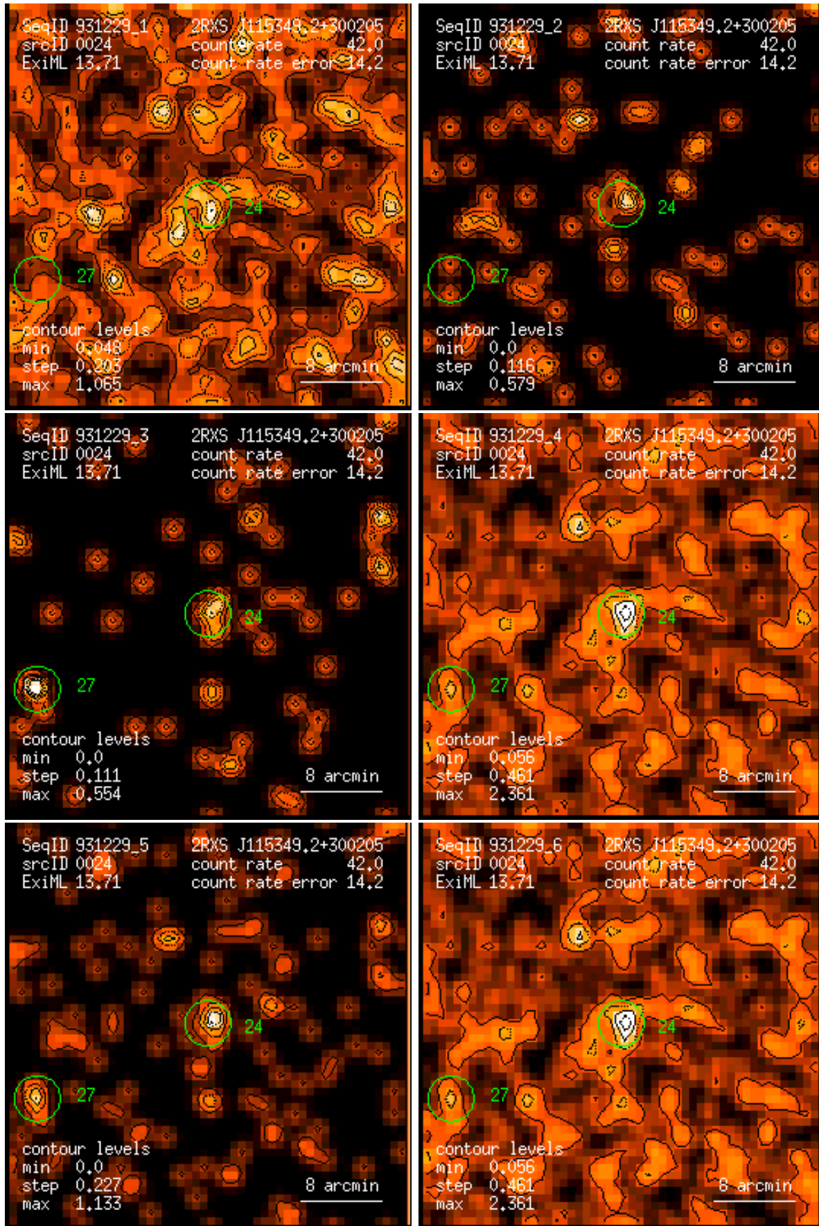
Figure 24: RASS 931229: detection 0024: band rate images, Gaussian filter: (1) PSPC channels 11 – 41, (2) 52 – 90, (3) 91 – 201, (4) 11 – 235, (5) 52 – 201, (6) 11 – 201. Broad band rates in counts/ks. Band rate contour levels in counts/ks/arcmin 2 .
