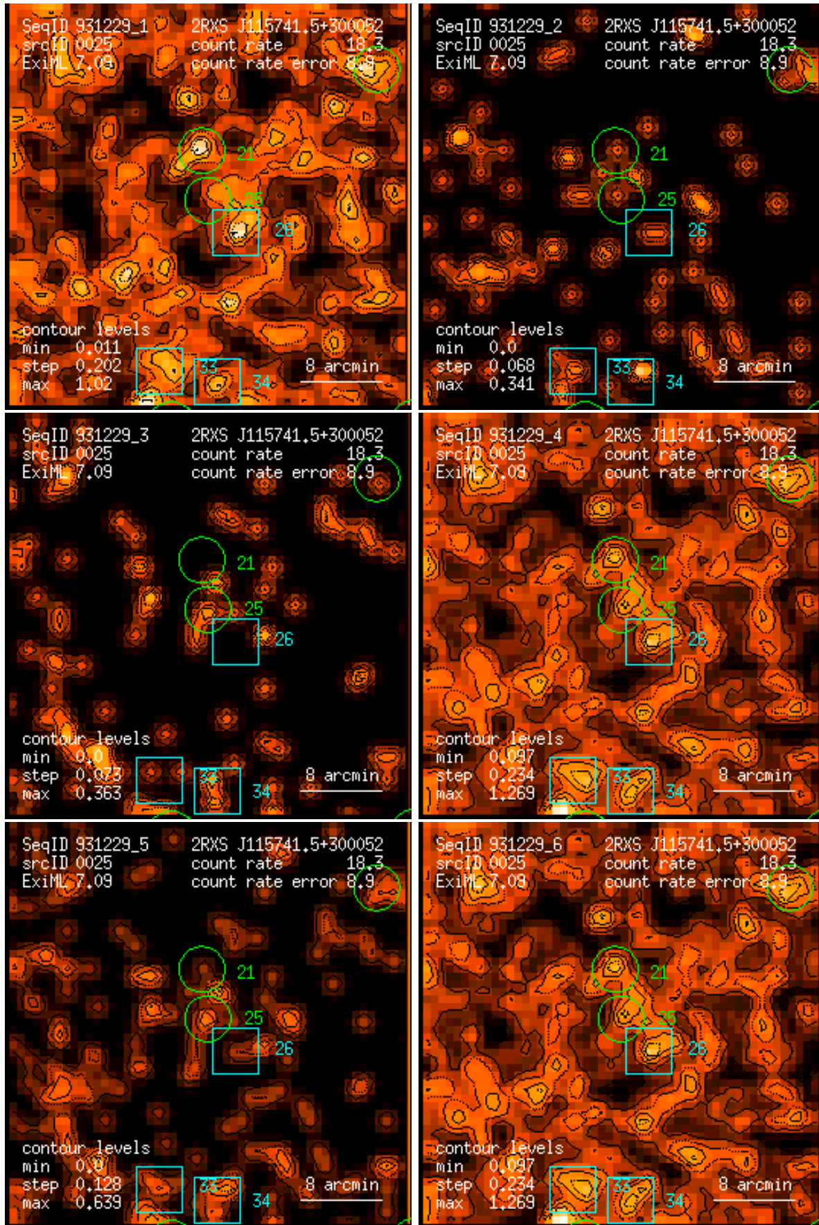
Figure 25: RASS 931229: detection 0025: band rate images, Gaussian filter: (1) PSPC channels 11 – 41, (2) 52 – 90, (3) 91 – 201, (4) 11 – 235, (5) 52 – 201, (6) 11 – 201. Broad band rates in counts/ks. Band rate contour levels in counts/ks/arcmin 2 .
