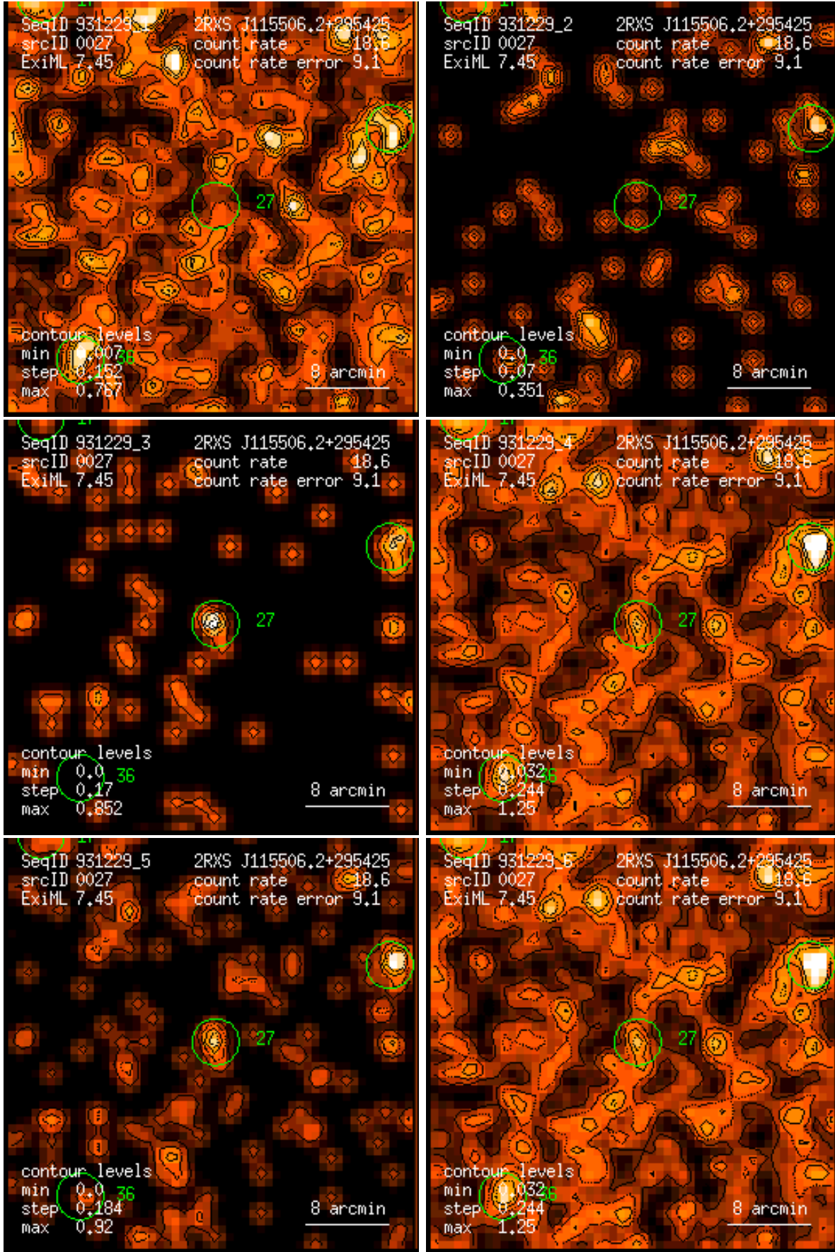
Figure 27: RASS 931229: detection 0027: band rate images, Gaussian filter: (1) PSPC channels 11 – 41, (2) 52 – 90, (3) 91 – 201, (4) 11 – 235, (5) 52 – 201, (6) 11 – 201. Broad band rates in counts/ks. Band rate contour levels in counts/ks/arcmin 2 .
