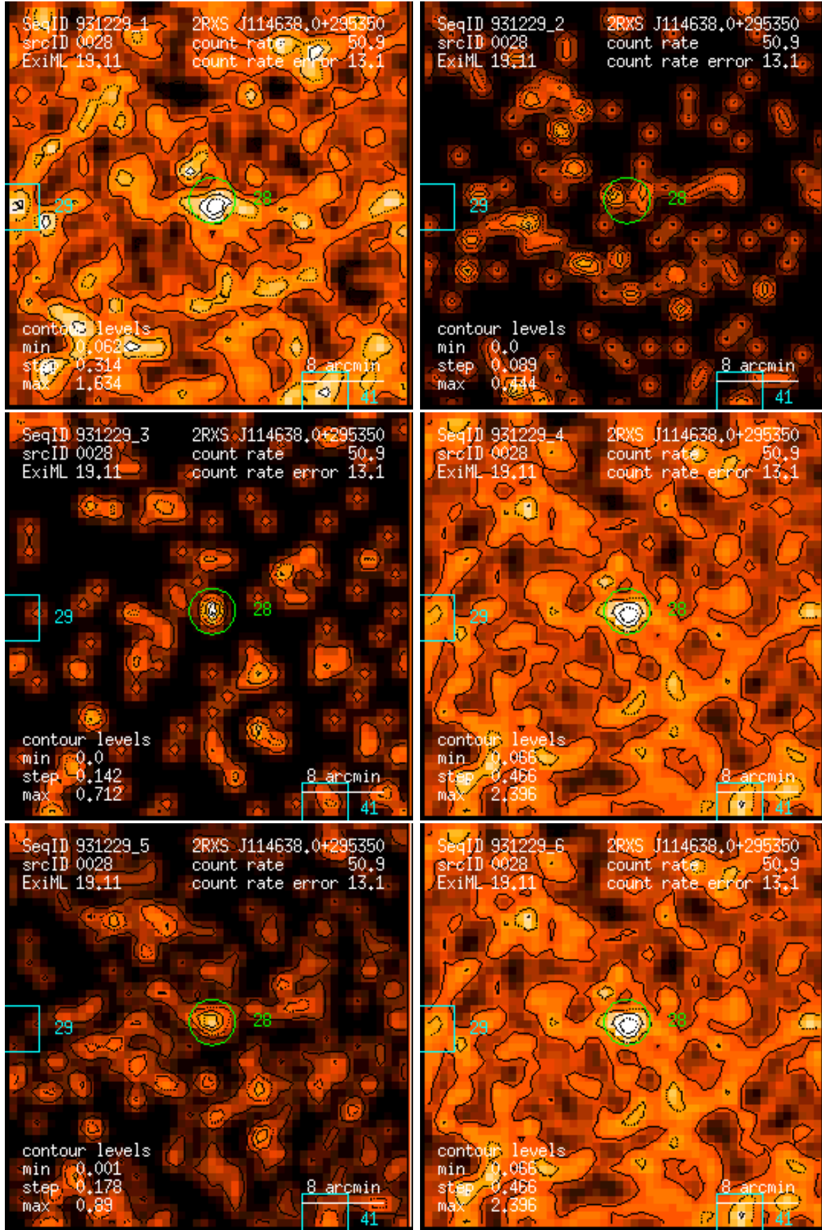
Figure 28: RASS 931229: detection 0028: band rate images, Gaussian filter: (1) PSPC channels 11 – 41, (2) 52 – 90, (3) 91 – 201, (4) 11 – 235, (5) 52 – 201, (6) 11 – 201. Broad band rates in counts/ks. Band rate contour levels in counts/ks/arcmin 2 .
