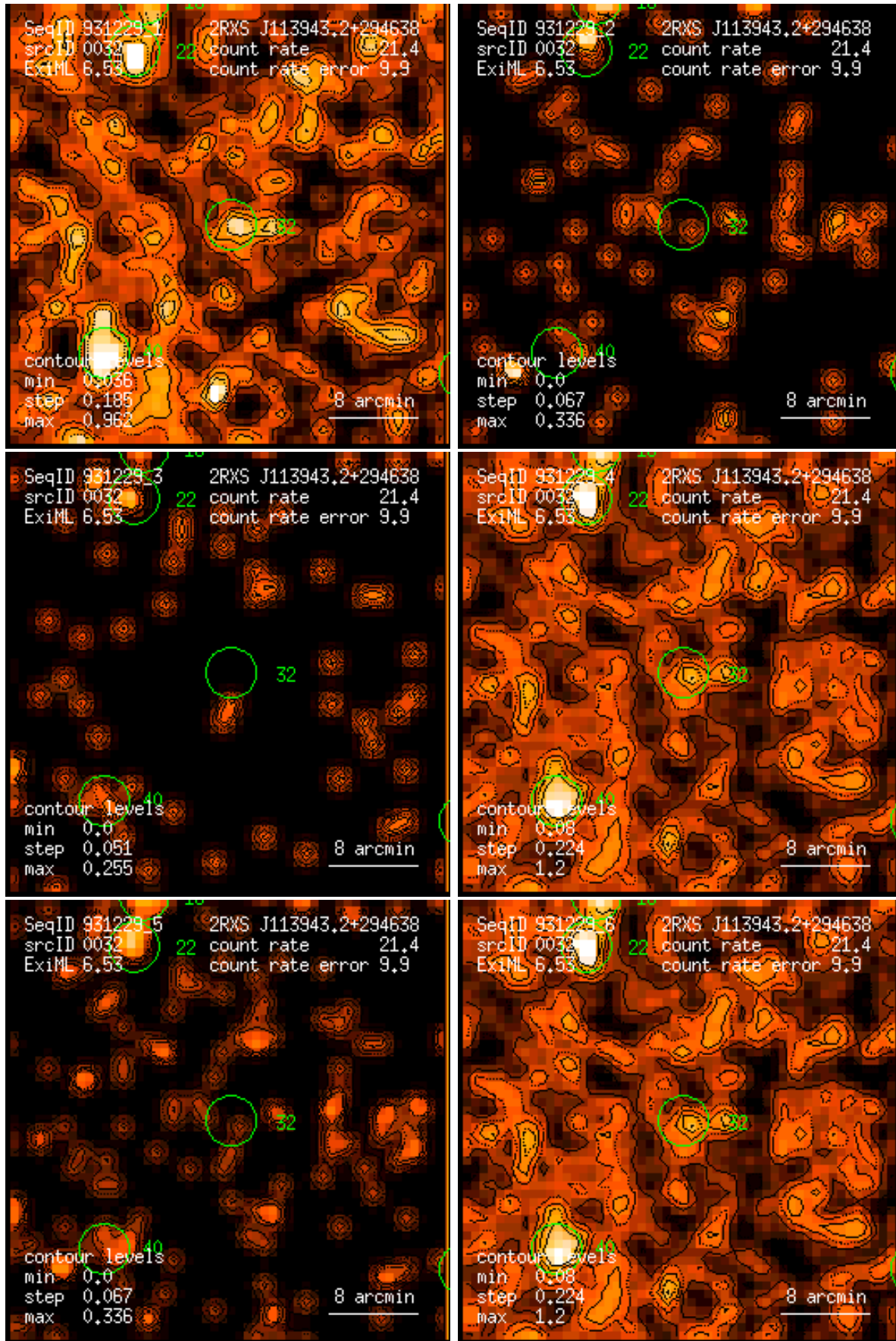
Figure 32: RASS 931229: detection 0032: band rate images, Gaussian filter: (1) PSPC channels 11 – 41, (2) 52 – 90, (3) 91 – 201, (4) 11 – 235, (5) 52 – 201, (6) 11 – 201. Broad band rates in counts/ks. Band rate contour levels in counts/ks/arcmin 2 .
