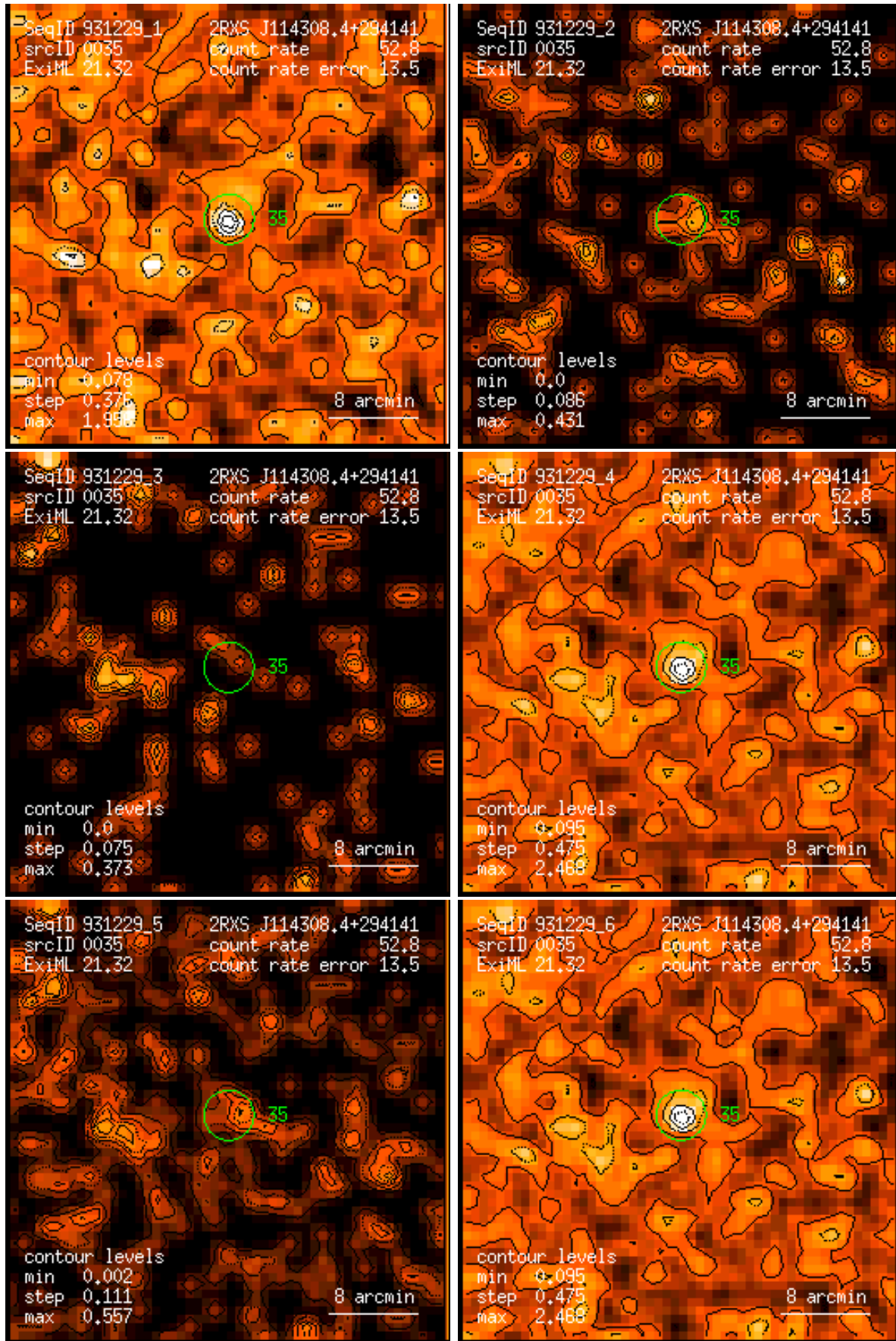
Figure 35: RASS 931229: detection 0035: band rate images, Gaussian filter: (1) PSPC channels 11 – 41, (2) 52 – 90, (3) 91 – 201, (4) 11 – 235, (5) 52 – 201, (6) 11 – 201. Broad band rates in counts/ks. Band rate contour levels in counts/ks/arcmin 2 .
