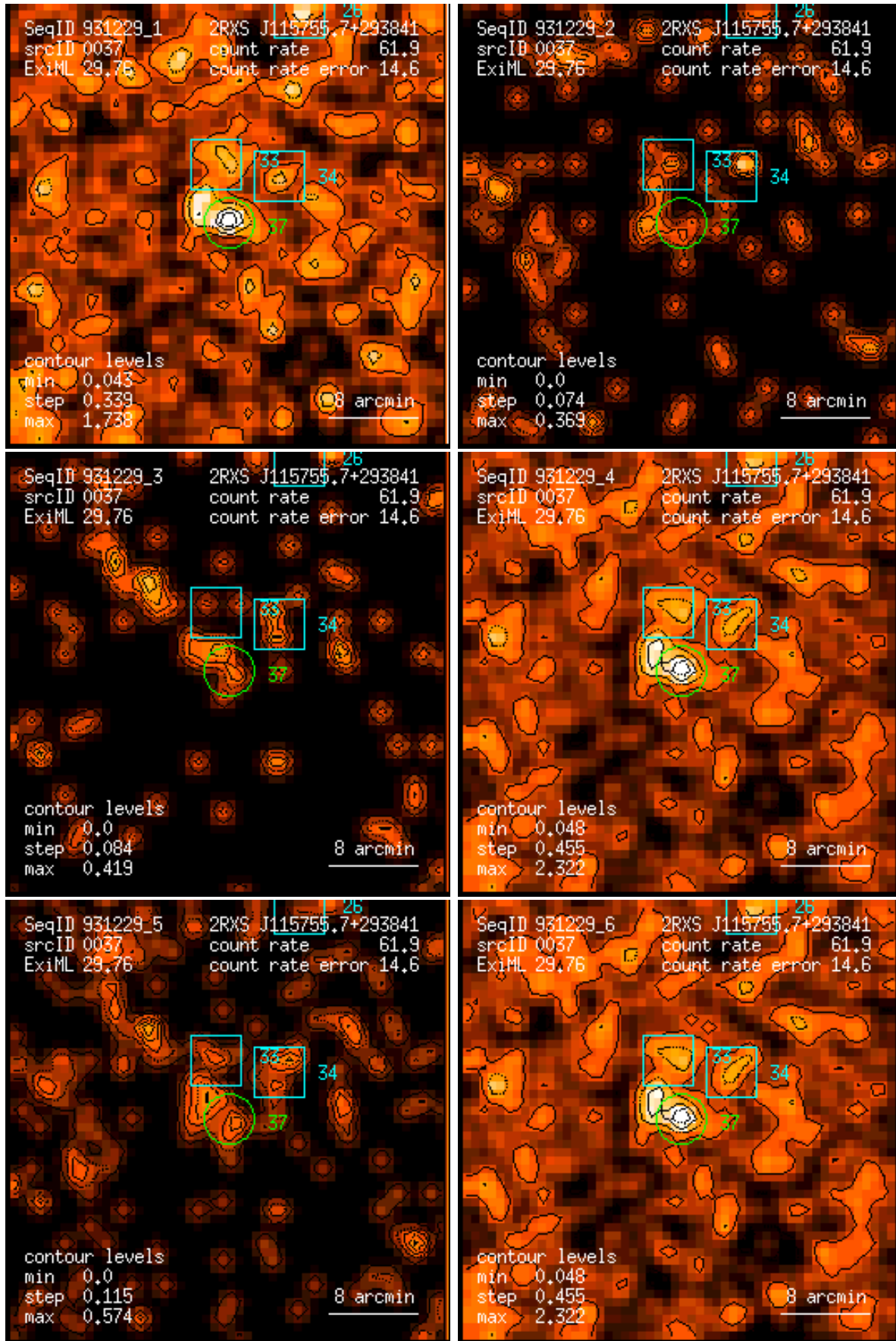
Figure 37: RASS 931229: detection 0037: band rate images, Gaussian filter: (1) PSPC channels 11 – 41, (2) 52 – 90, (3) 91 – 201, (4) 11 – 235, (5) 52 – 201, (6) 11 – 201. Broad band rates in counts/ks. Band rate contour levels in counts/ks/arcmin 2 .
