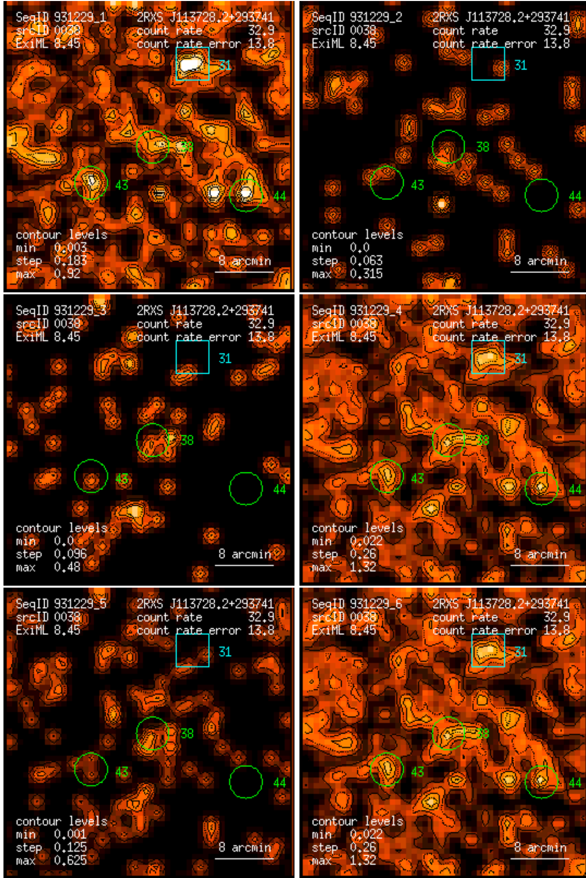
Figure 38: RASS 931229: detection 0038: band rate images, Gaussian filter: (1) PSPC channels 11 – 41, (2) 52 – 90, (3) 91 – 201, (4) 11 – 235, (5) 52 – 201, (6) 11 – 201. Broad band rates in counts/ks. Band rate contour levels in counts/ks/arcmin 2 .
