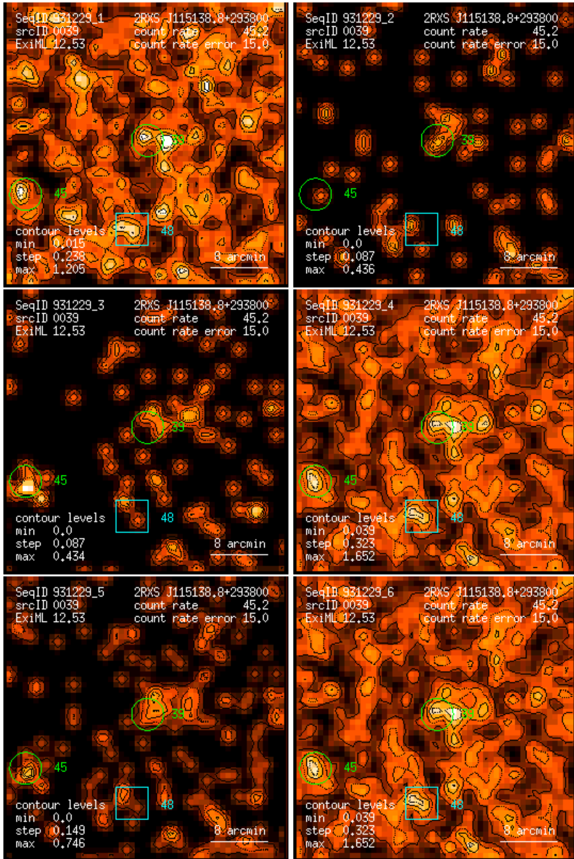
Figure 39: RASS 931229: detection 0039: band rate images, Gaussian filter: (1) PSPC channels 11 – 41, (2) 52 – 90, (3) 91 – 201, (4) 11 – 235, (5) 52 – 201, (6) 11 – 201. Broad band rates in counts/ks. Band rate contour levels in counts/ks/arcmin 2 .
