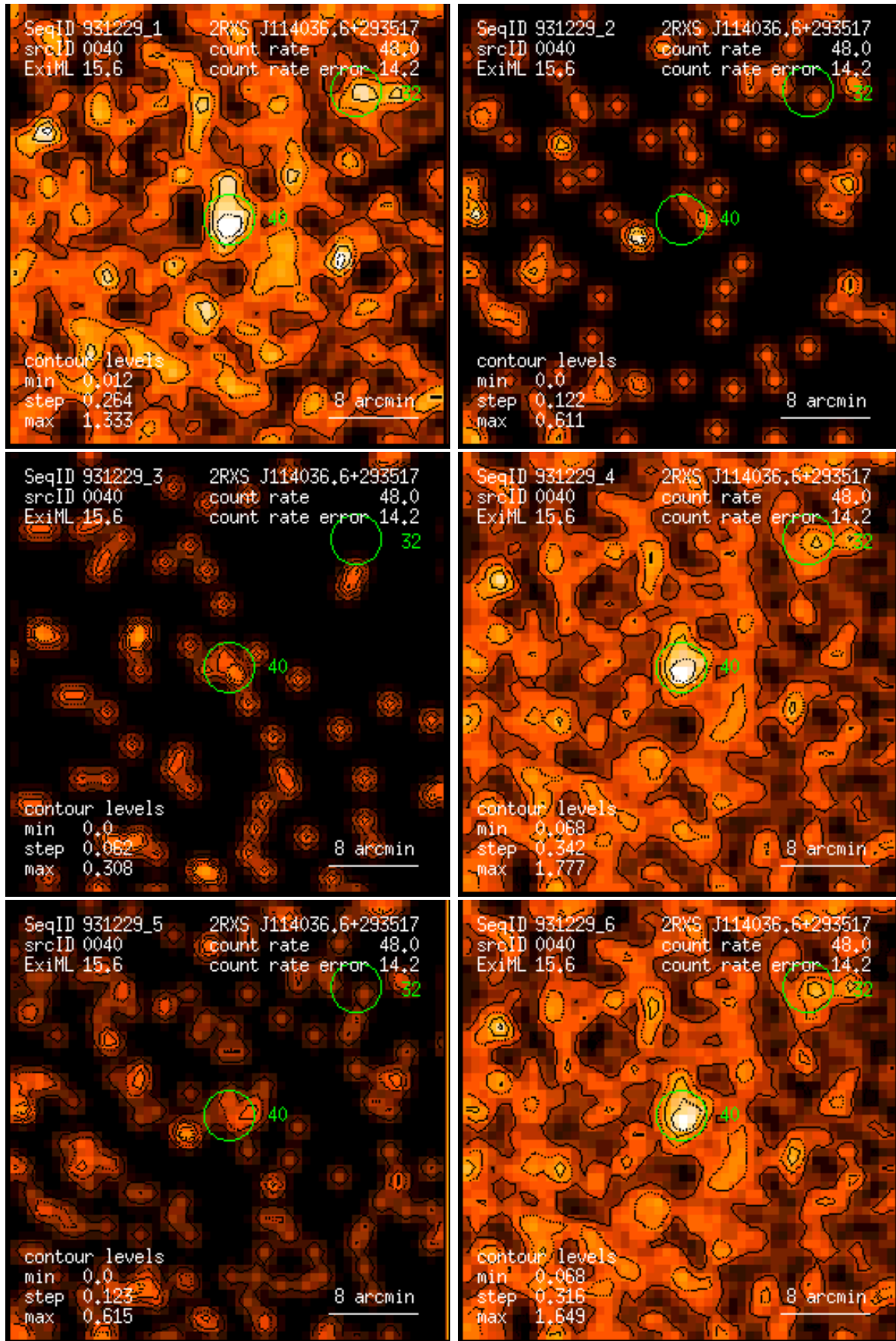
Figure 40: RASS 931229: detection 0040: band rate images, Gaussian filter: (1) PSPC channels 11 – 41, (2) 52 – 90, (3) 91 – 201, (4) 11 – 235, (5) 52 – 201, (6) 11 – 201. Broad band rates in counts/ks. Band rate contour levels in counts/ks/arcmin 2 .
