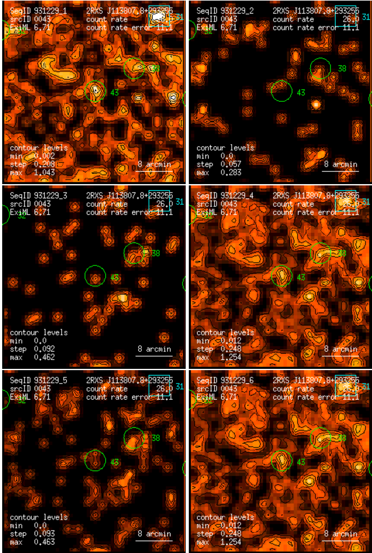
Figure 43: RASS 931229: detection 0043: band rate images, Gaussian filter: (1) PSPC channels 11 – 41, (2) 52 – 90, (3) 91 – 201, (4) 11 – 235, (5) 52 – 201, (6) 11 – 201. Broad band rates in counts/ks. Band rate contour levels in counts/ks/arcmin 2 .
