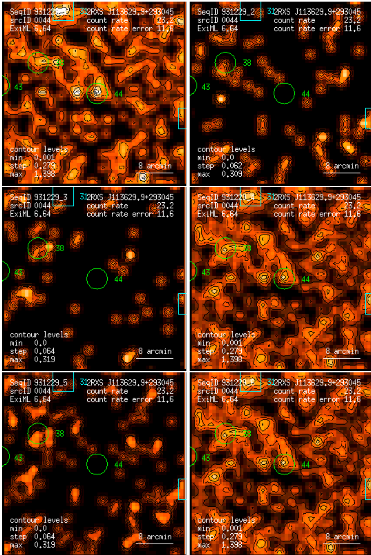
Figure 44: RASS 931229: detection 0044: band rate images, Gaussian filter: (1) PSPC channels 11 – 41, (2) 52 – 90, (3) 91 – 201, (4) 11 – 235, (5) 52 – 201, (6) 11 – 201. Broad band rates in counts/ks. Band rate contour levels in counts/ks/arcmin 2 .
