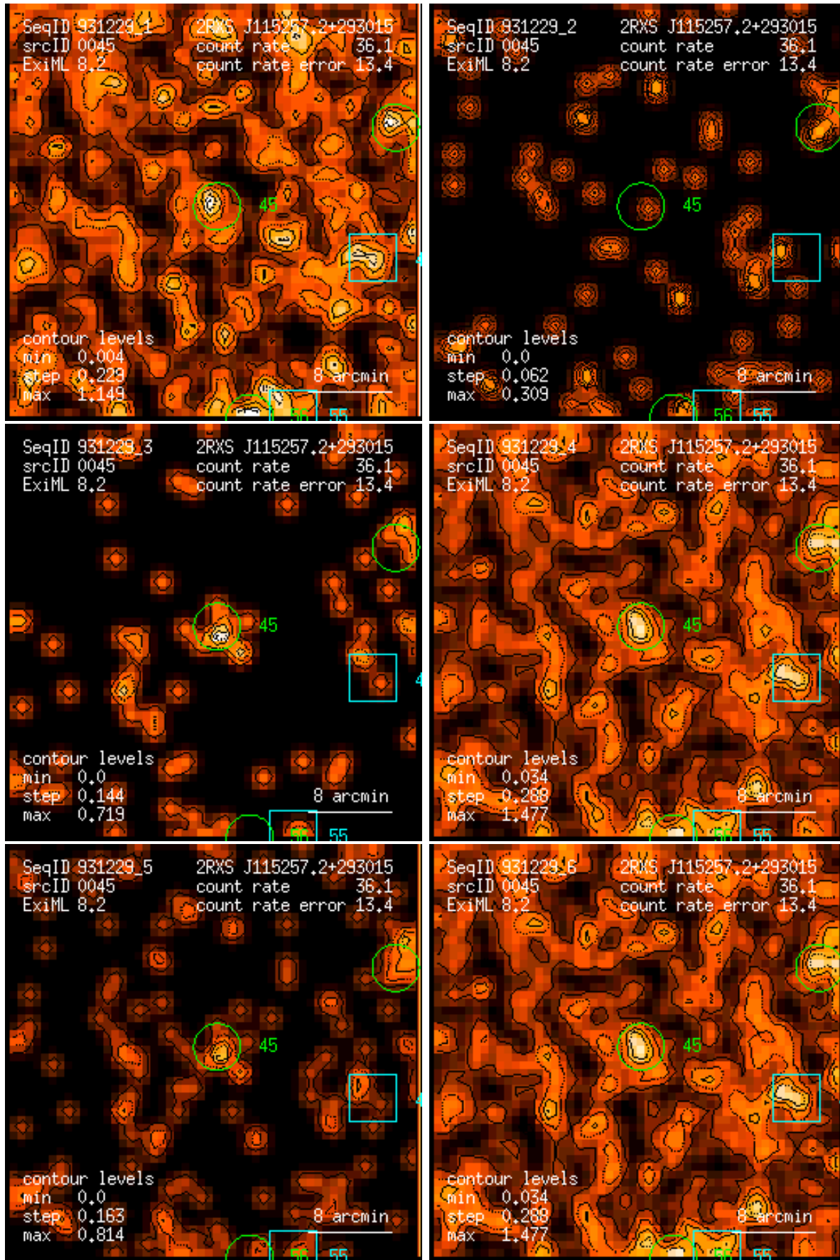
Figure 45: RASS 931229: detection 0045: band rate images, Gaussian filter: (1) PSPC channels 11 – 41, (2) 52 – 90, (3) 91 – 201, (4) 11 – 235, (5) 52 – 201, (6) 11 – 201. Broad band rates in counts/ks. Band rate contour levels in counts/ks/arcmin 2 .
