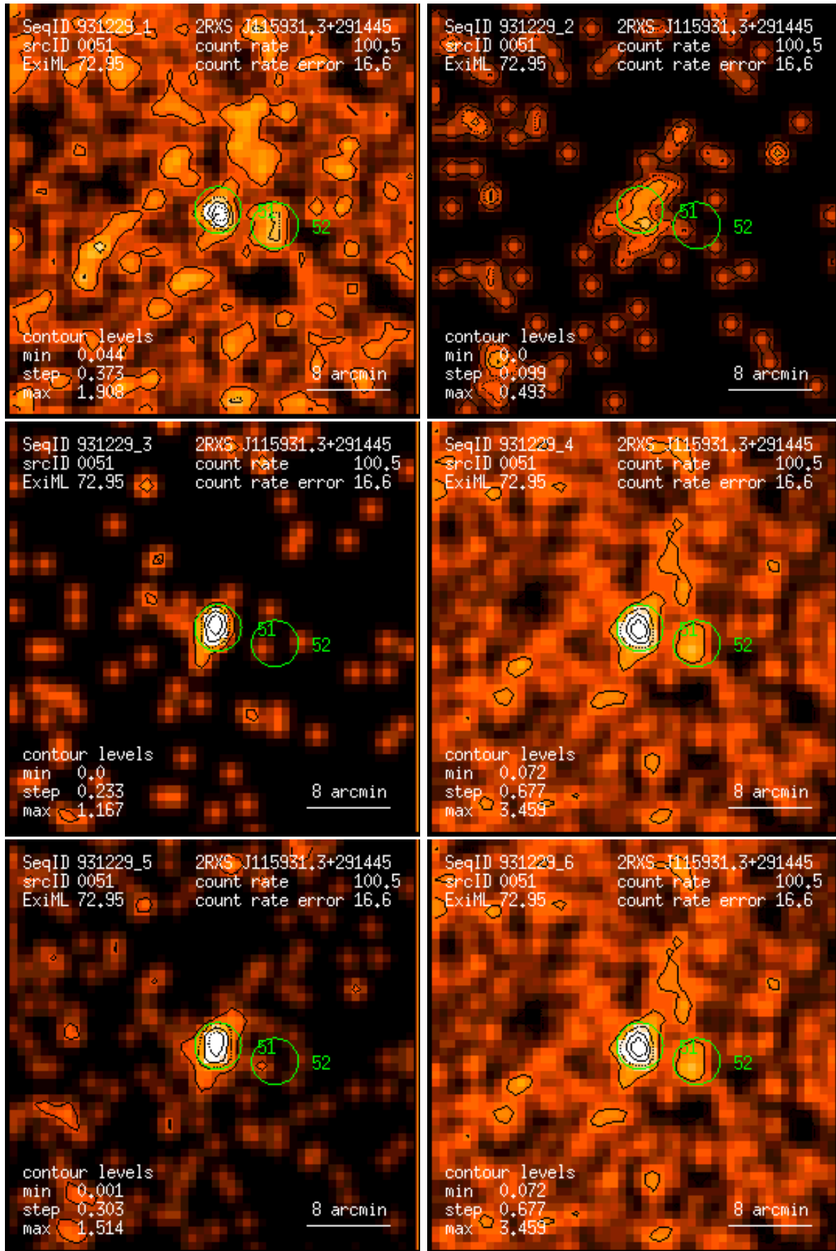
Figure 51: RASS 931229: detection 0051: band rate images, Gaussian filter: (1) PSPC channels 11 – 41, (2) 52 – 90, (3) 91 – 201, (4) 11 – 235, (5) 52 – 201, (6) 11 – 201. Broad band rates in counts/ks. Band rate contour levels in counts/ks/arcmin 2 .
