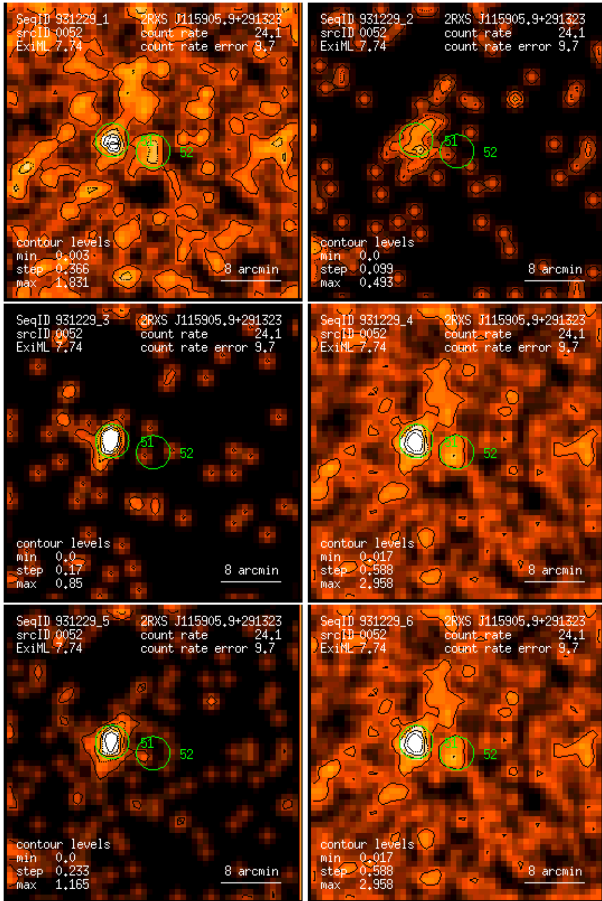
Figure 52: RASS 931229: detection 0052: band rate images, Gaussian filter: (1) PSPC channels 11 – 41, (2) 52 – 90, (3) 91 – 201, (4) 11 – 235, (5) 52 – 201, (6) 11 – 201. Broad band rates in counts/ks. Band rate contour levels in counts/ks/arcmin 2 .
