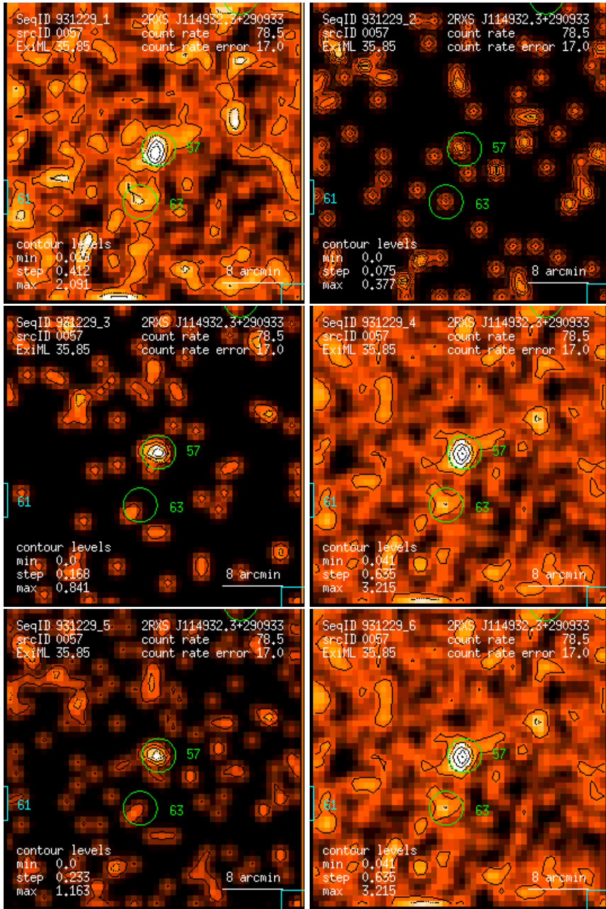
Figure 57: RASS 931229: detection 0057: band rate images, Gaussian filter: (1) PSPC channels 11 – 41, (2) 52 – 90, (3) 91 – 201, (4) 11 – 235, (5) 52 – 201, (6) 11 – 201. Broad band rates in counts/ks. Band rate contour levels in counts/ks/arcmin 2 .
