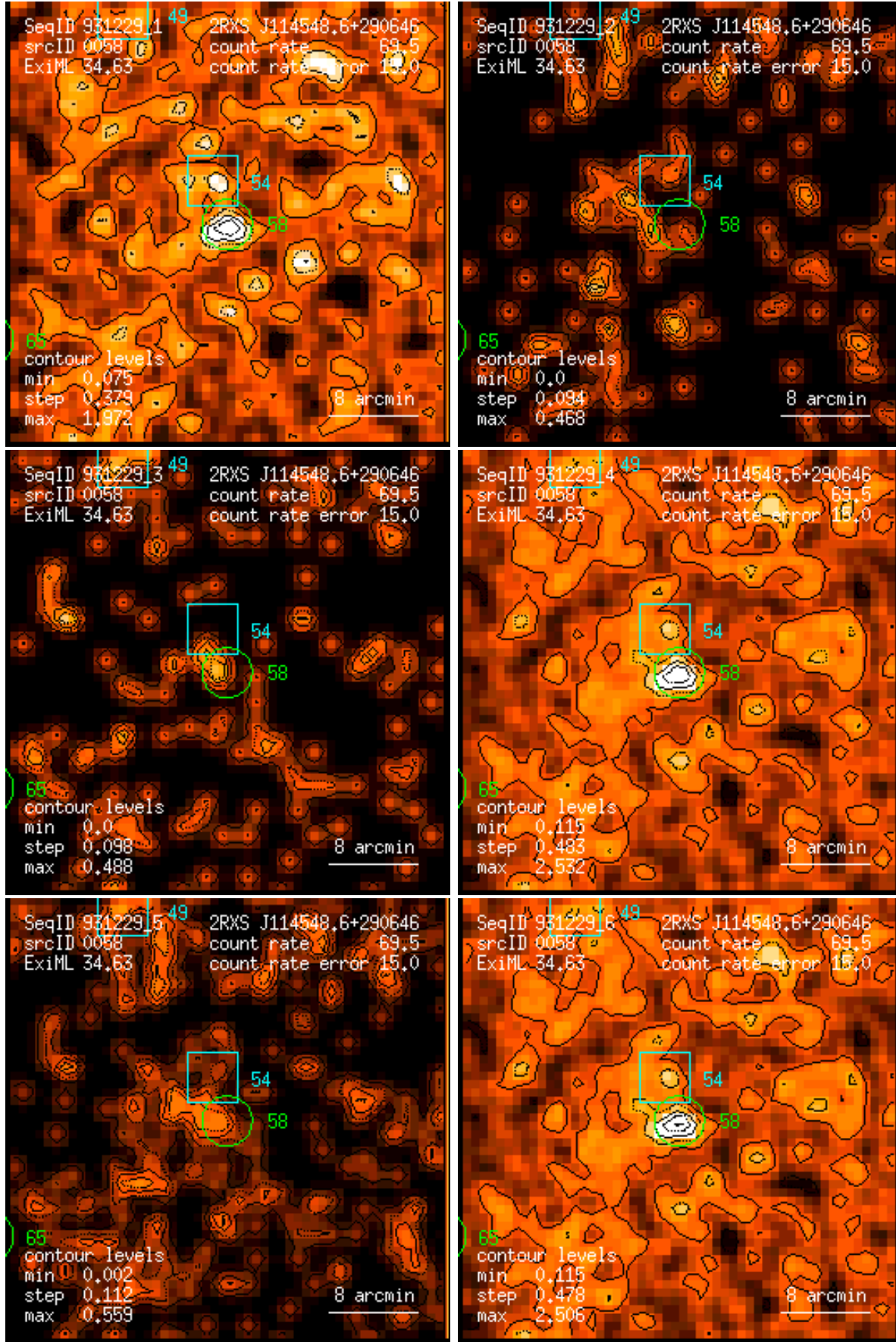
Figure 58: RASS 931229: detection 0058: band rate images, Gaussian filter: (1) PSPC channels 11 – 41, (2) 52 – 90, (3) 91 – 201, (4) 11 – 235, (5) 52 – 201, (6) 11 – 201. Broad band rates in counts/ks. Band rate contour levels in counts/ks/arcmin 2 .
