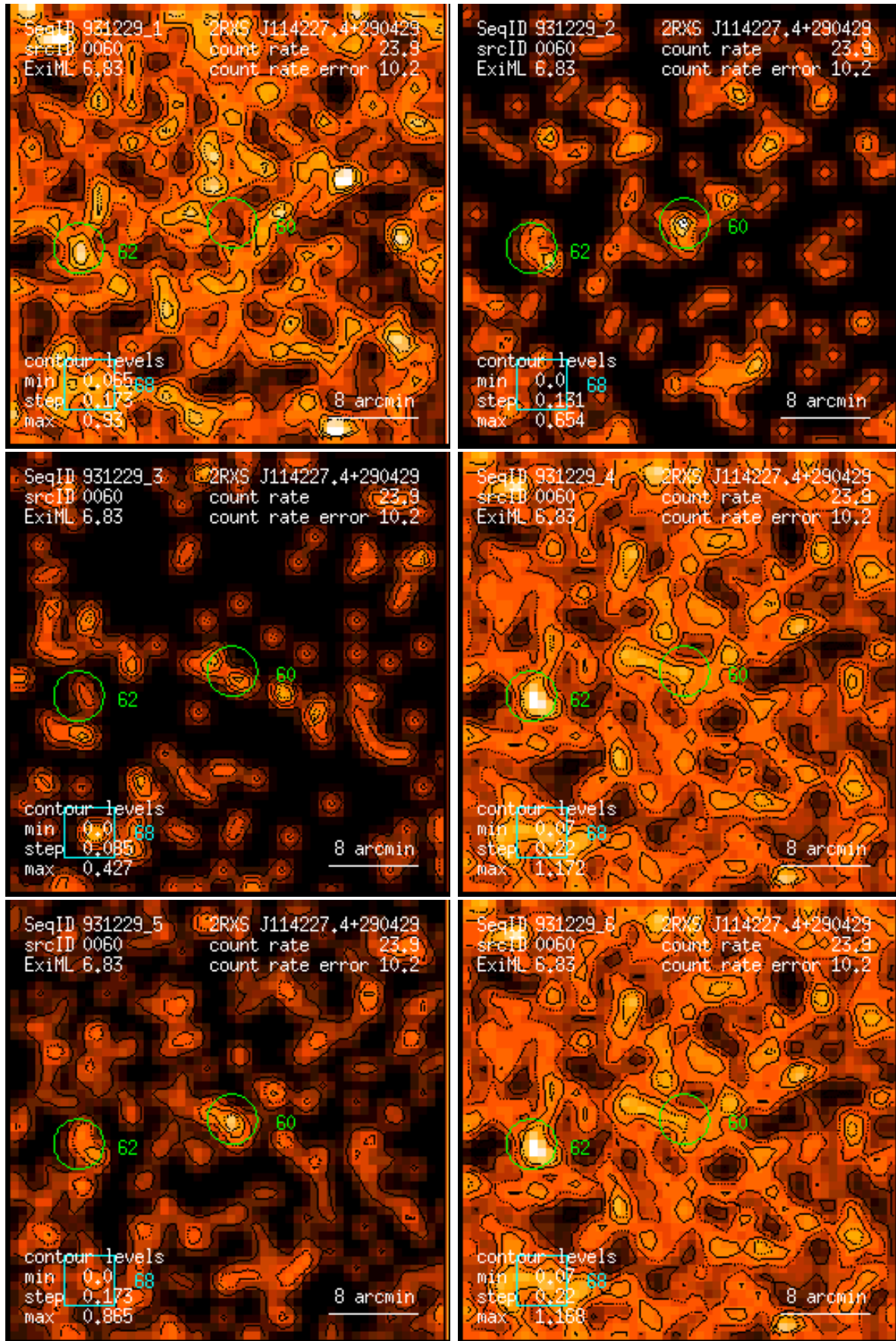
Figure 60: RASS 931229: detection 0060: band rate images, Gaussian filter: (1) PSPC channels 11 – 41, (2) 52 – 90, (3) 91 – 201, (4) 11 – 235, (5) 52 – 201, (6) 11 – 201. Broad band rates in counts/ks. Band rate contour levels in counts/ks/arcmin 2 .
