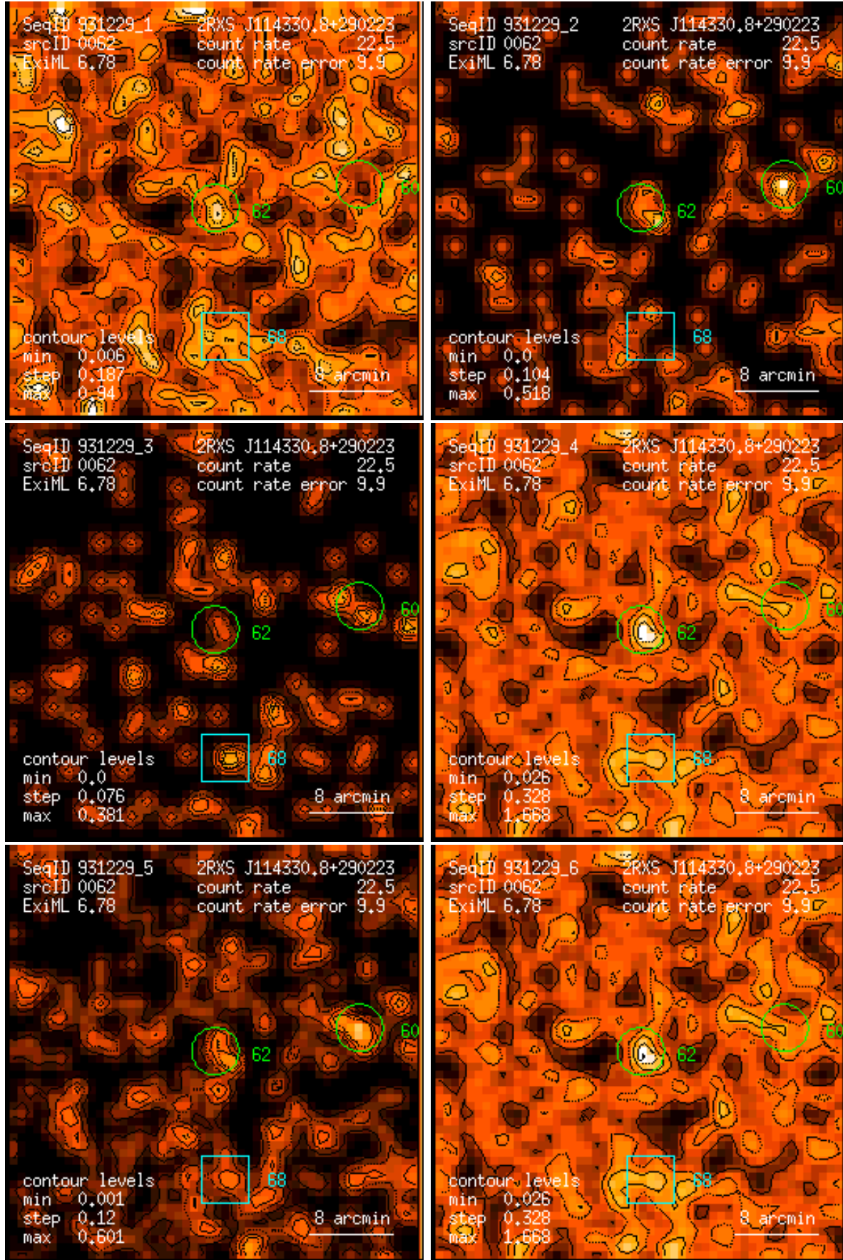
Figure 62: RASS 931229: detection 0062: band rate images, Gaussian filter: (1) PSPC channels 11 – 41, (2) 52 – 90, (3) 91 – 201, (4) 11 – 235, (5) 52 – 201, (6) 11 – 201. Broad band rates in counts/ks. Band rate contour levels in counts/ks/arcmin 2 .
