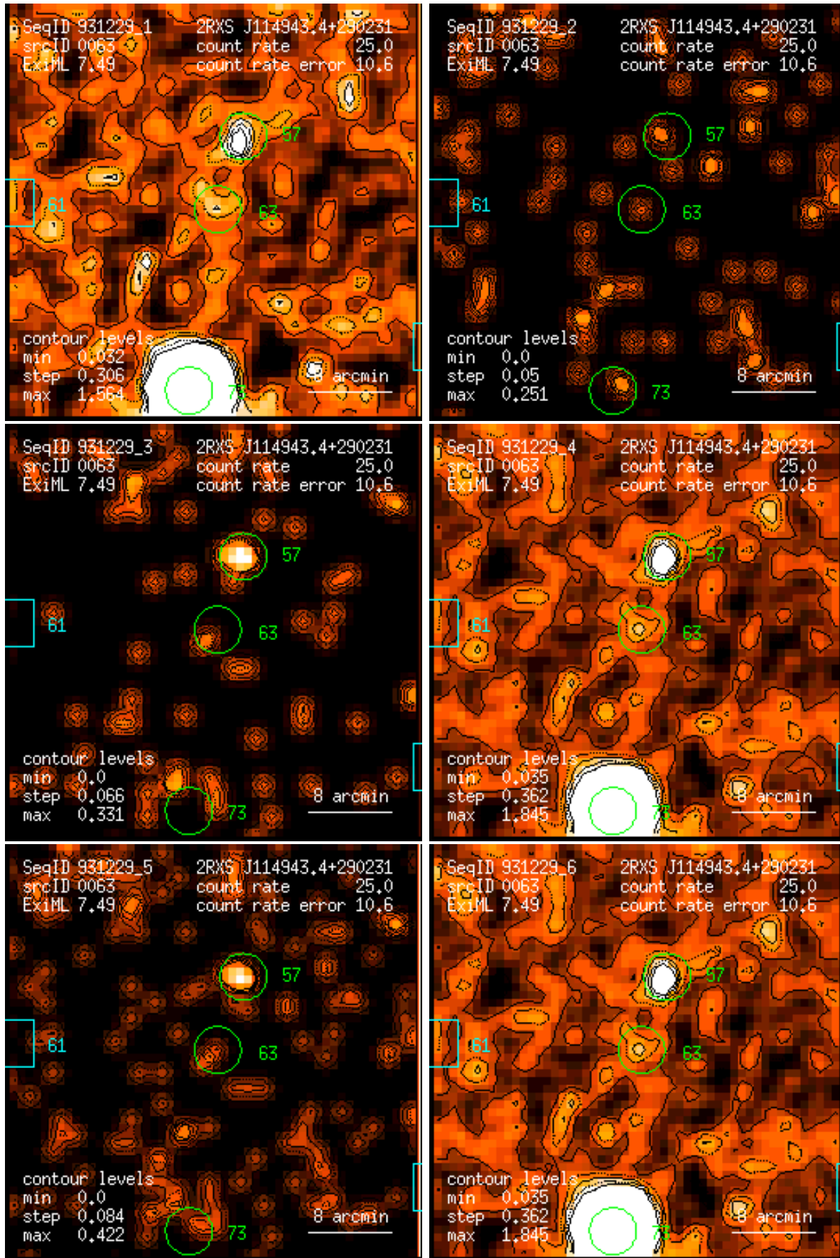
Figure 63: RASS 931229: detection 0063: band rate images, Gaussian filter: (1) PSPC channels 11 – 41, (2) 52 – 90, (3) 91 – 201, (4) 11 – 235, (5) 52 – 201, (6) 11 – 201. Broad band rates in counts/ks. Band rate contour levels in counts/ks/arcmin 2 .
