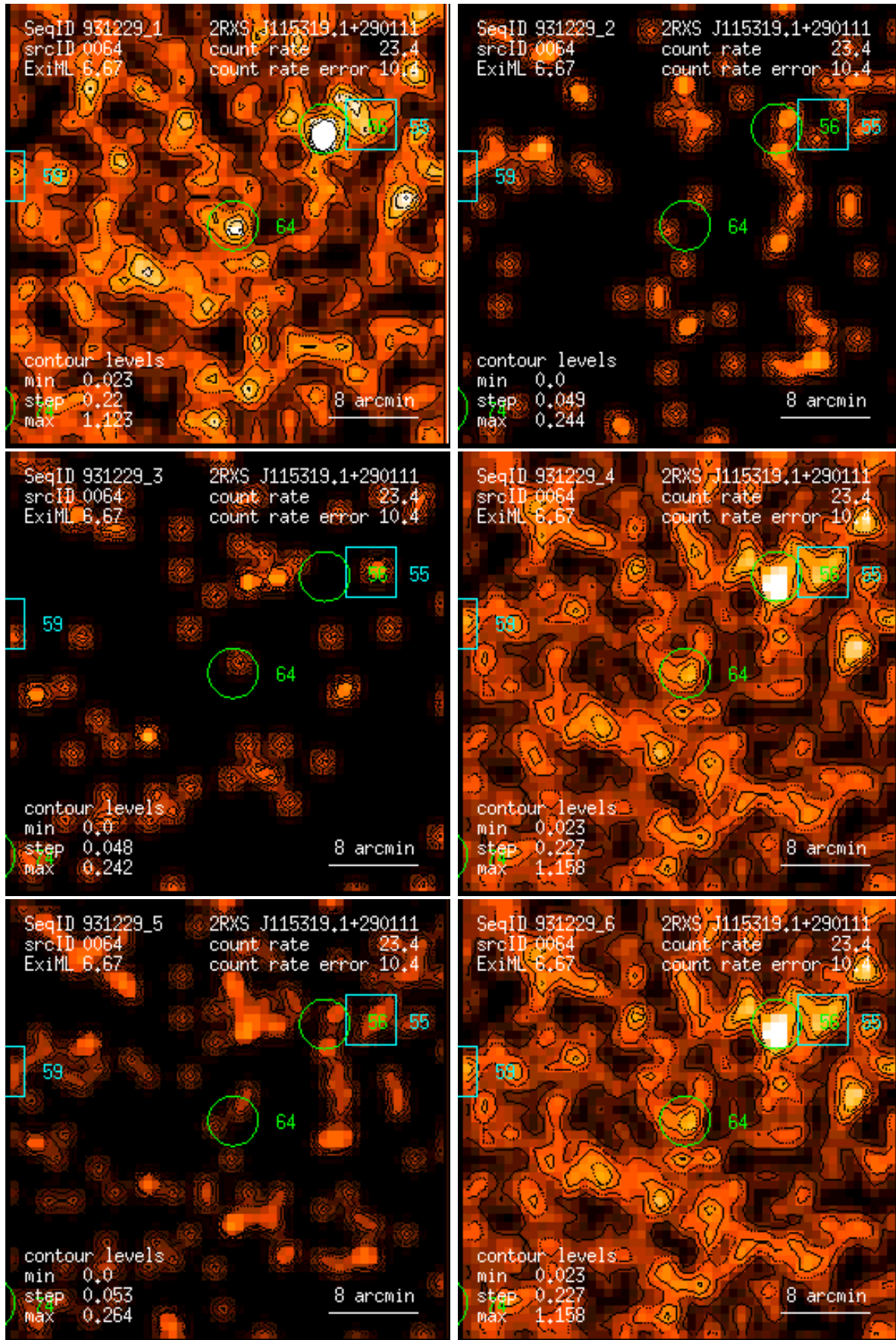
Figure 64: RASS 931229: detection 0064: band rate images, Gaussian filter: (1) PSPC channels 11 – 41, (2) 52 – 90, (3) 91 – 201, (4) 11 – 235, (5) 52 – 201, (6) 11 – 201. Broad band rates in counts/ks. Band rate contour levels in counts/ks/arcmin 2 .
