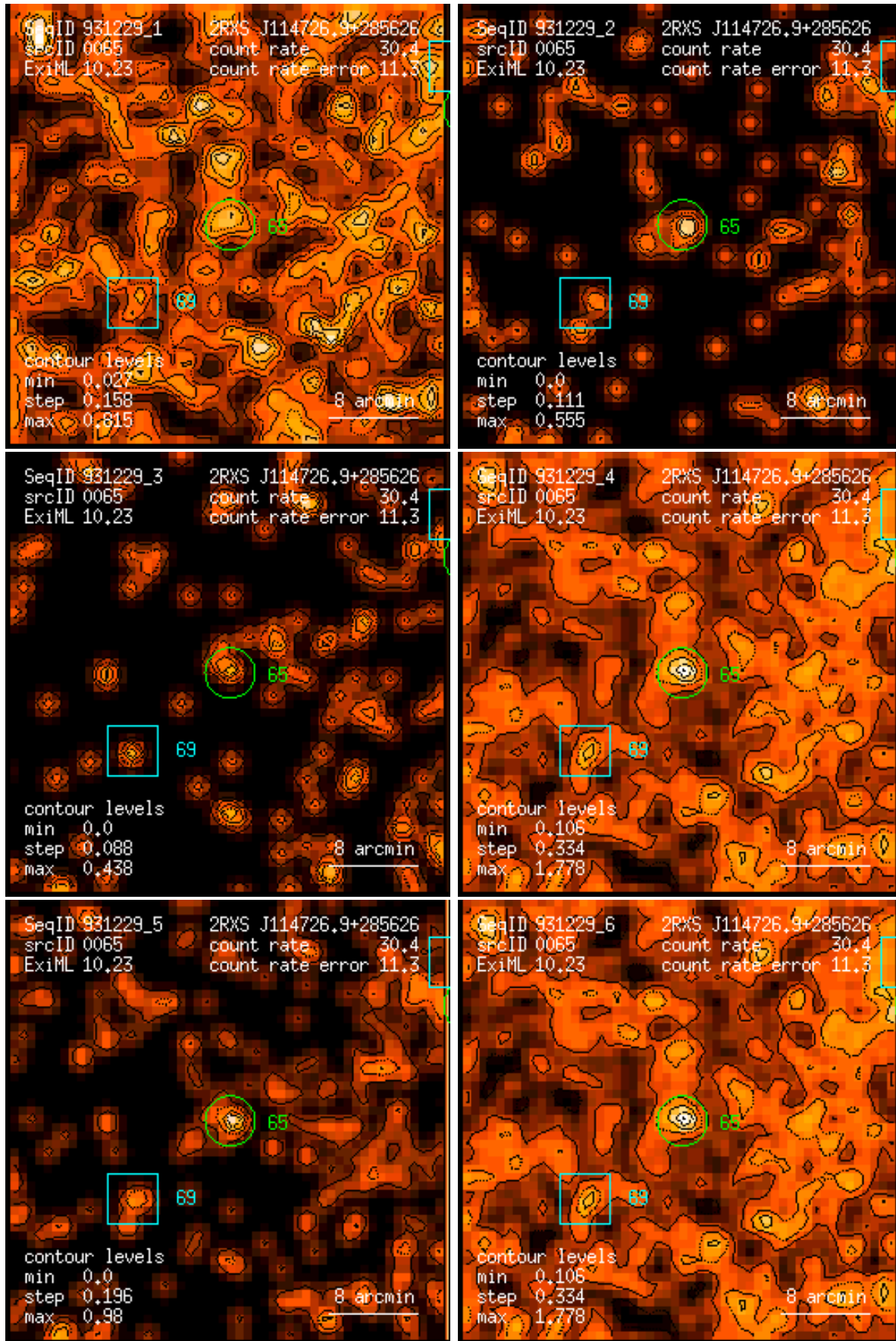
Figure 65: RASS 931229: detection 0065: band rate images, Gaussian filter: (1) PSPC channels 11 – 41, (2) 52 – 90, (3) 91 – 201, (4) 11 – 235, (5) 52 – 201, (6) 11 – 201. Broad band rates in counts/ks. Band rate contour levels in counts/ks/arcmin 2 .
