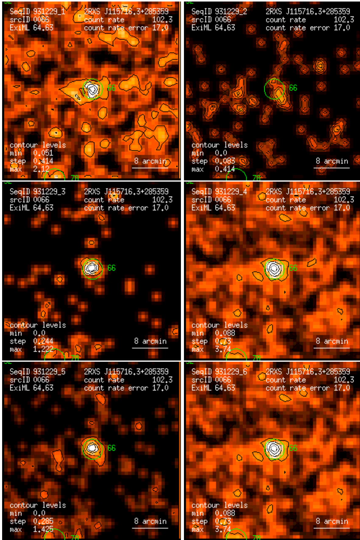
Figure 66: RASS 931229: detection 0066: band rate images, Gaussian filter: (1) PSPC channels 11 – 41, (2) 52 – 90, (3) 91 – 201, (4) 11 – 235, (5) 52 – 201, (6) 11 – 201. Broad band rates in counts/ks. Band rate contour levels in counts/ks/arcmin 2 .
