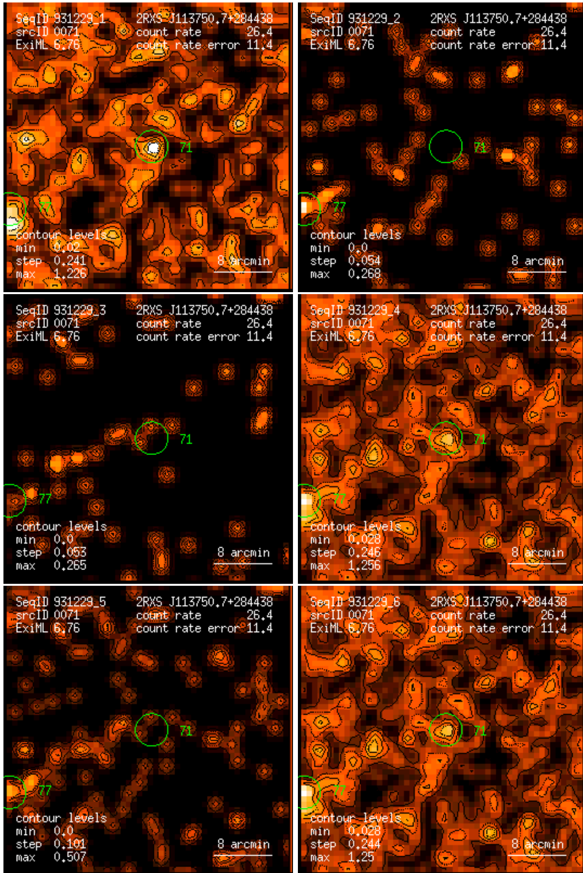
Figure 71: RASS 931229: detection 0071: band rate images, Gaussian filter: (1) PSPC channels 11 – 41, (2) 52 – 90, (3) 91 – 201, (4) 11 – 235, (5) 52 – 201, (6) 11 – 201. Broad band rates in counts/ks. Band rate contour levels in counts/ks/arcmin 2 .
