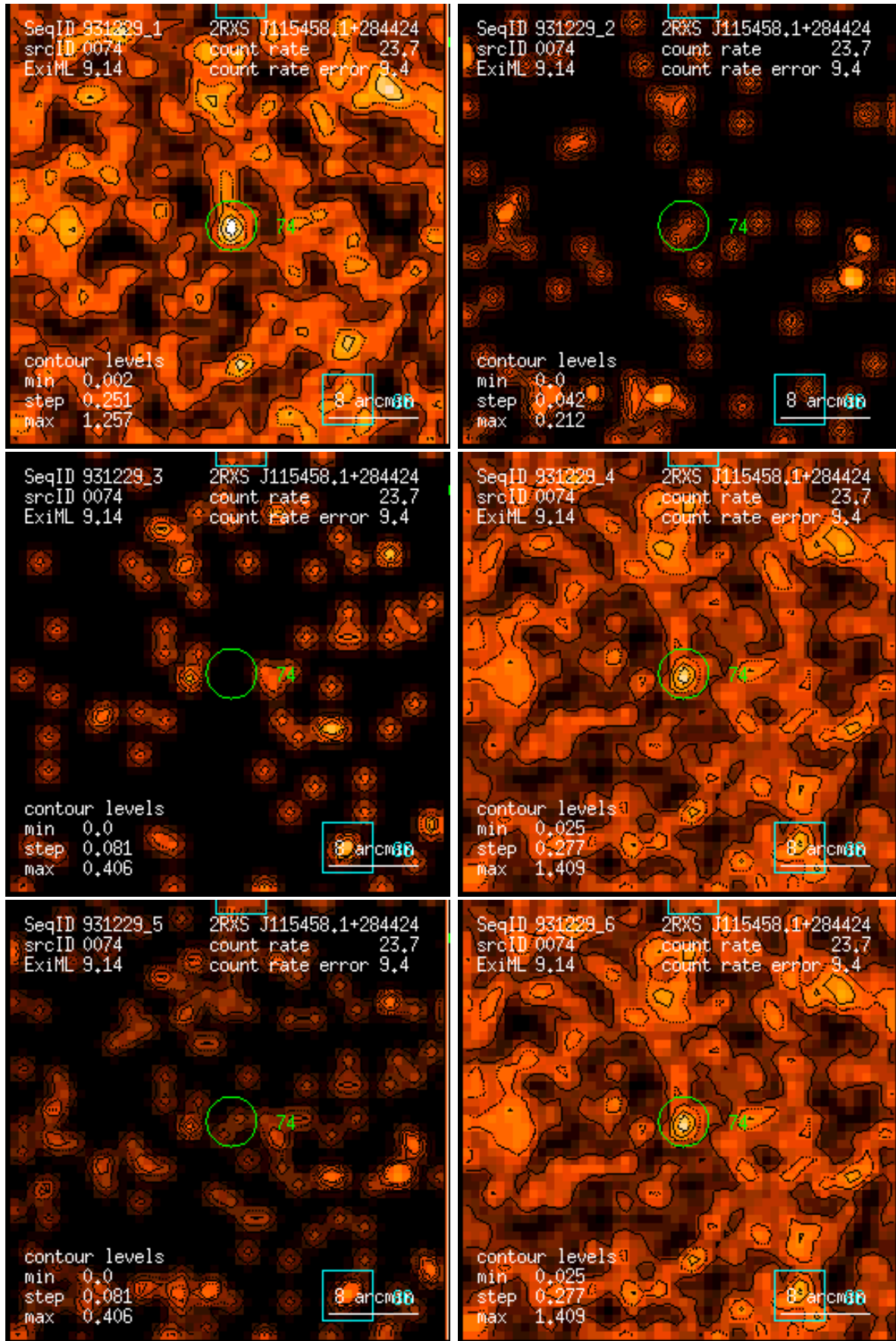
Figure 74: RASS 931229: detection 0074: band rate images, Gaussian filter: (1) PSPC channels 11 – 41, (2) 52 – 90, (3) 91 – 201, (4) 11 – 235, (5) 52 – 201, (6) 11 – 201. Broad band rates in counts/ks. Band rate contour levels in counts/ks/arcmin 2 .
