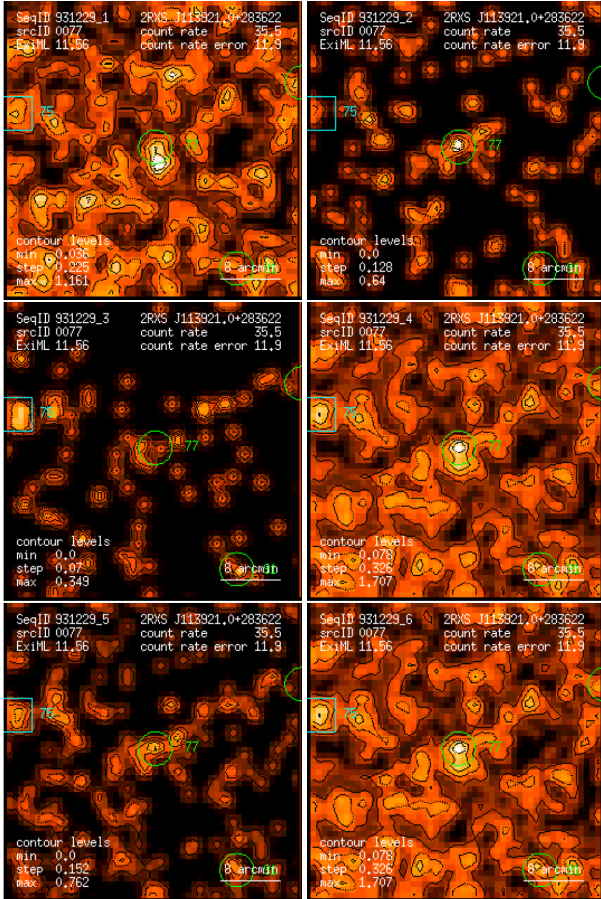
Figure 77: RASS 931229: detection 0077: band rate images, Gaussian filter: (1) PSPC channels 11 – 41, (2) 52 – 90, (3) 91 – 201, (4) 11 – 235, (5) 52 – 201, (6) 11 – 201. Broad band rates in counts/ks. Band rate contour levels in counts/ks/arcmin 2 .
