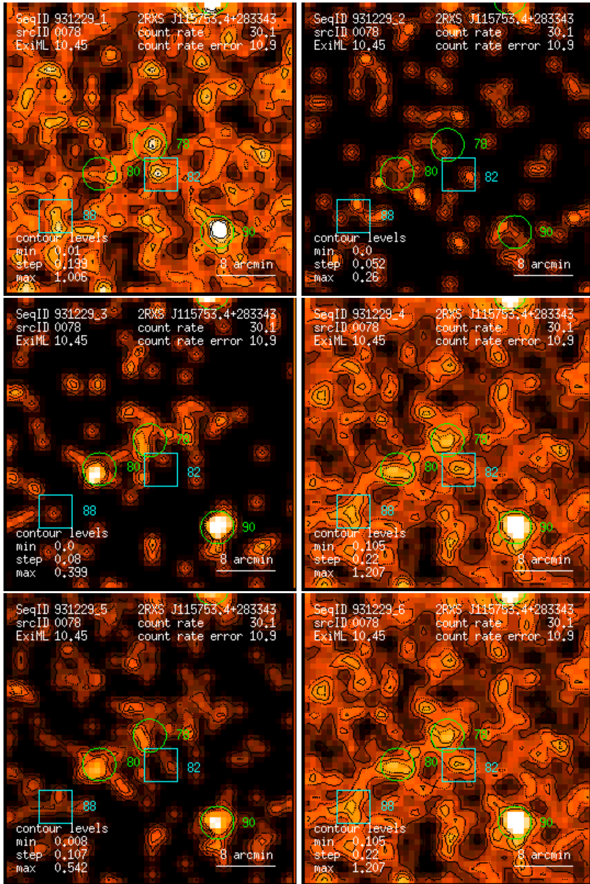
Figure 78: RASS 931229: detection 0078: band rate images, Gaussian filter: (1) PSPC channels 11 – 41, (2) 52 – 90, (3) 91 – 201, (4) 11 – 235, (5) 52 – 201, (6) 11 – 201. Broad band rates in counts/ks. Band rate contour levels in counts/ks/arcmin 2 .
