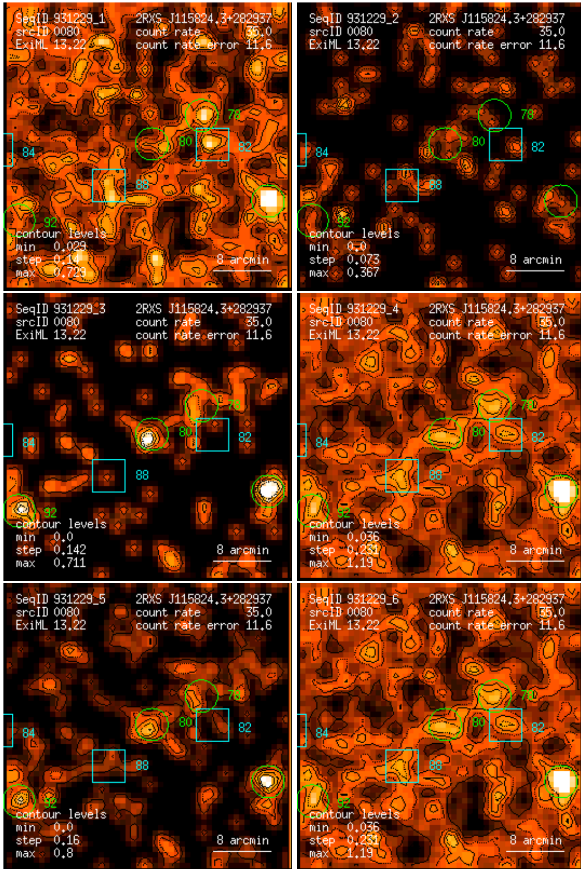
Figure 80: RASS 931229: detection 0080: band rate images, Gaussian filter: (1) PSPC channels 11 – 41, (2) 52 – 90, (3) 91 – 201, (4) 11 – 235, (5) 52 – 201, (6) 11 – 201. Broad band rates in counts/ks. Band rate contour levels in counts/ks/arcmin 2 .
