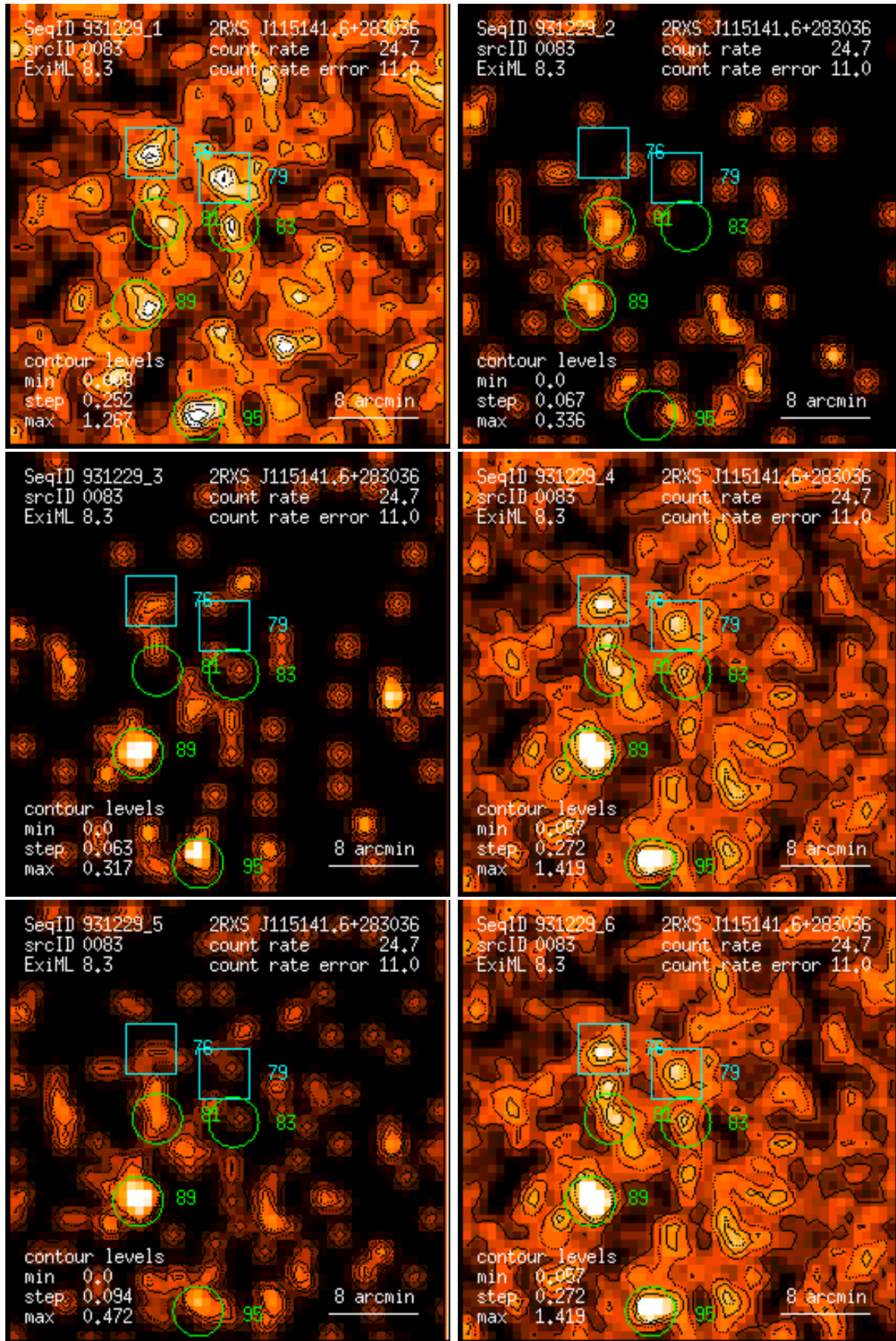
Figure 83: RASS 931229: detection 0083: band rate images, Gaussian filter: (1) PSPC channels 11 – 41, (2) 52 – 90, (3) 91 – 201, (4) 11 – 235, (5) 52 – 201, (6) 11 – 201. Broad band rates in counts/ks. Band rate contour levels in counts/ks/arcmin 2 .
