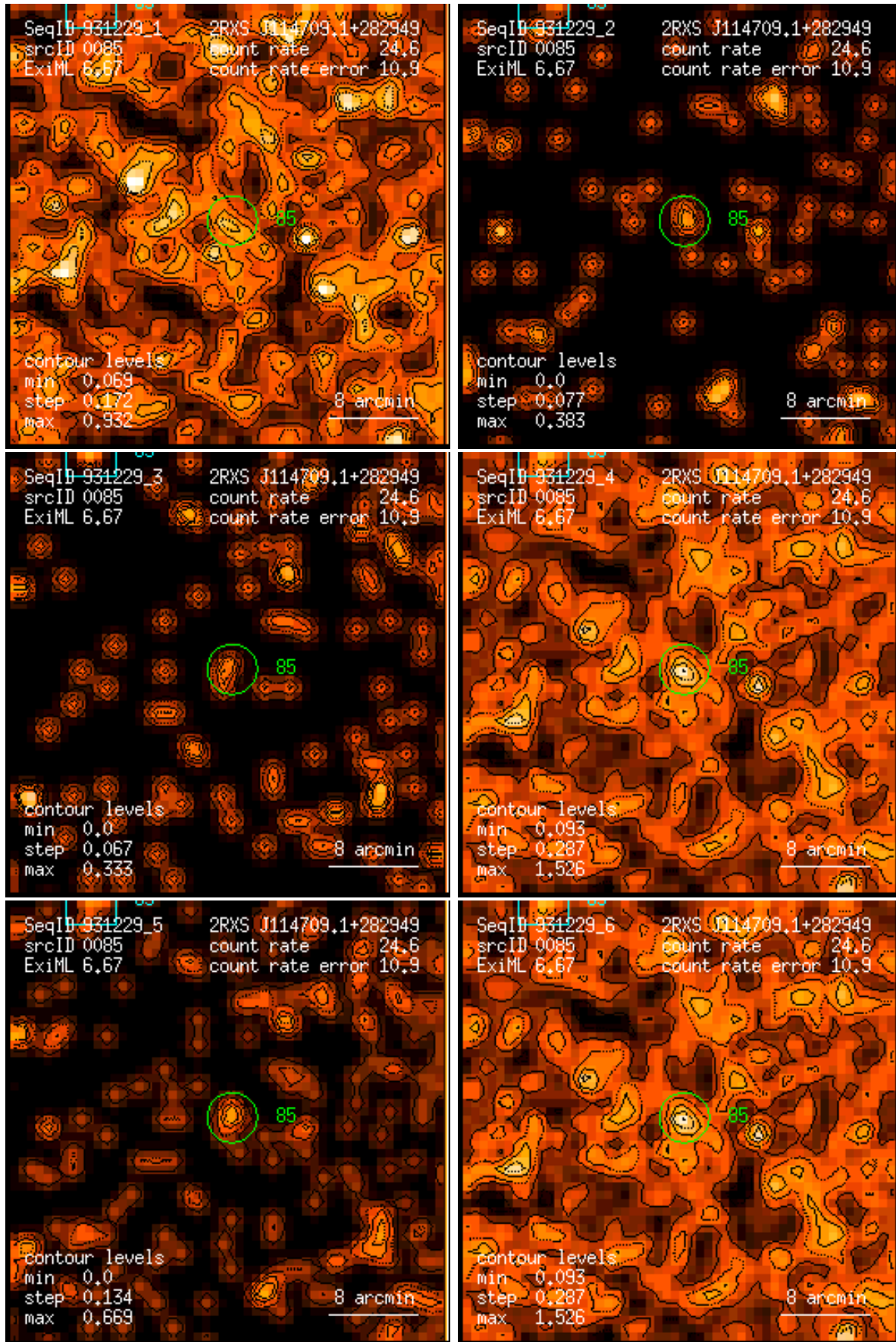
Figure 85: RASS 931229: detection 0085: band rate images, Gaussian filter: (1) PSPC channels 11 – 41, (2) 52 – 90, (3) 91 – 201, (4) 11 – 235, (5) 52 – 201, (6) 11 – 201. Broad band rates in counts/ks. Band rate contour levels in counts/ks/arcmin 2 .
