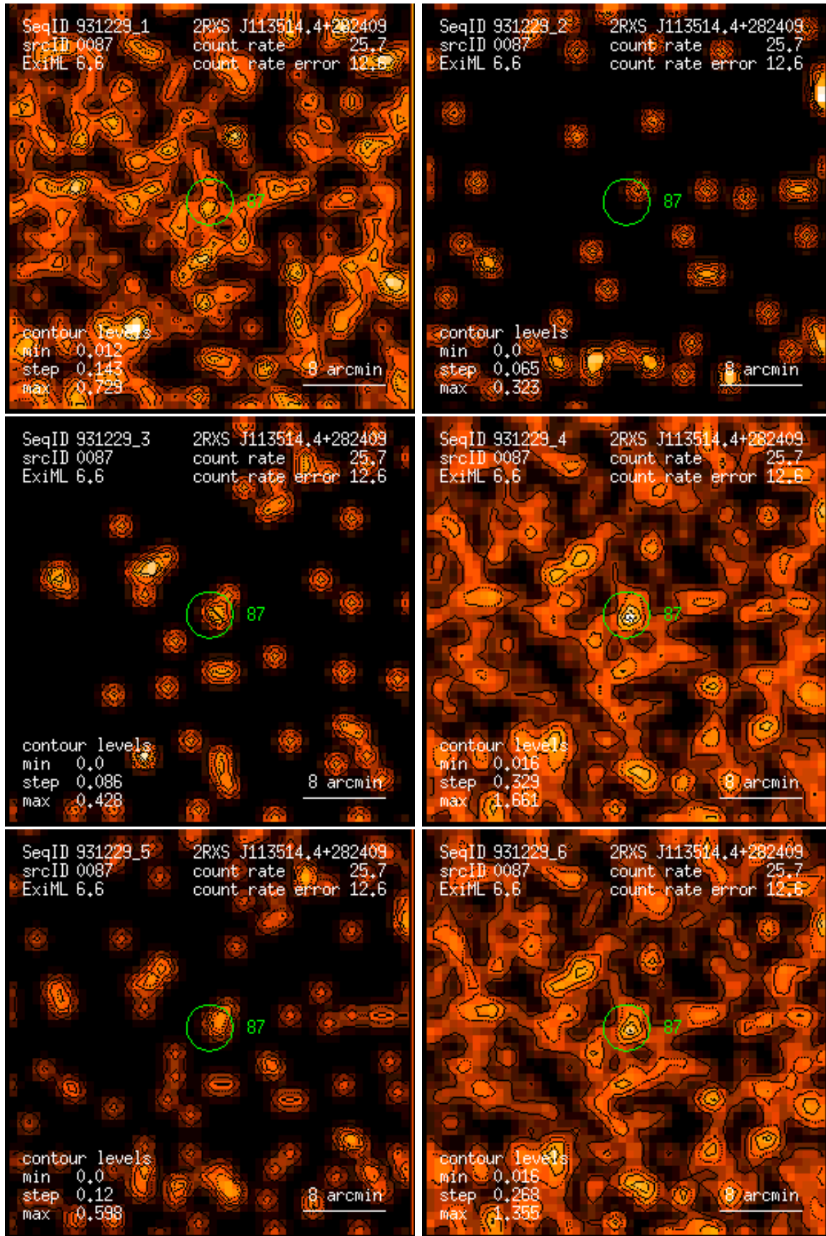
Figure 87: RASS 931229: detection 0087: band rate images, Gaussian filter: (1) PSPC channels 11 – 41, (2) 52 – 90, (3) 91 – 201, (4) 11 – 235, (5) 52 – 201, (6) 11 – 201. Broad band rates in counts/ks. Band rate contour levels in counts/ks/arcmin 2 .
