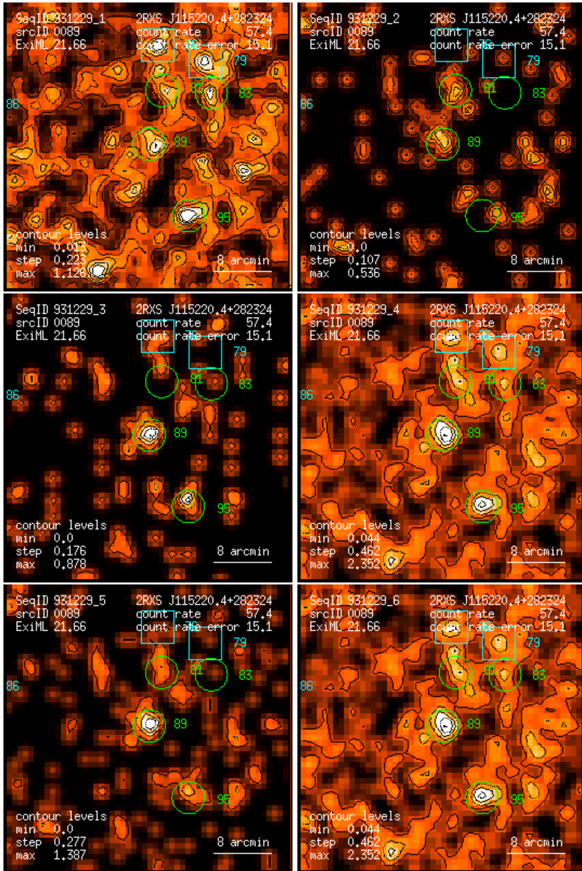
Figure 89: RASS 931229: detection 0089: band rate images, Gaussian filter: (1) PSPC channels 11 – 41, (2) 52 – 90, (3) 91 – 201, (4) 11 – 235, (5) 52 – 201, (6) 11 – 201. Broad band rates in counts/ks. Band rate contour levels in counts/ks/arcmin 2 .
