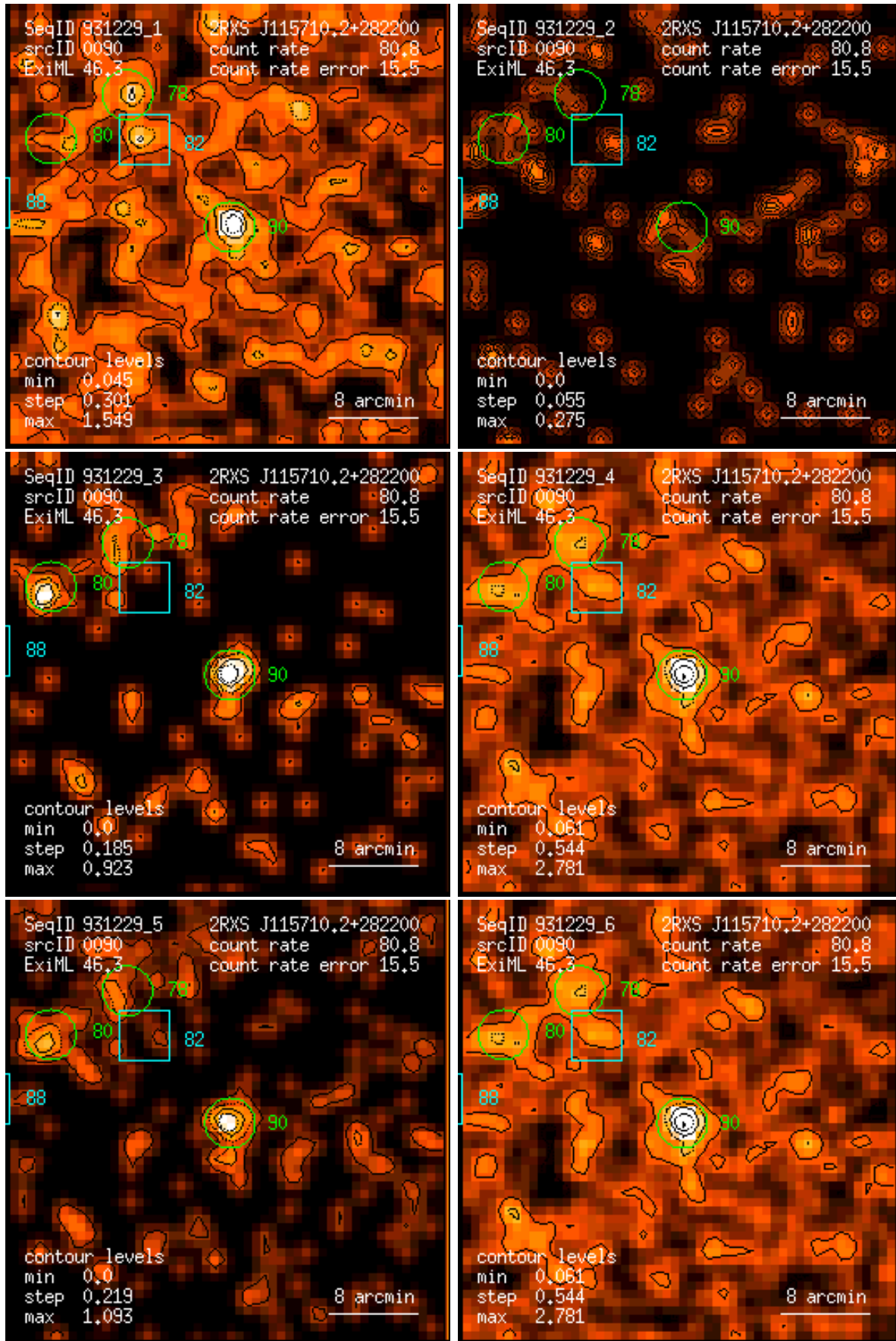
Figure 90: RASS 931229: detection 0090: band rate images, Gaussian filter: (1) PSPC channels 11 – 41, (2) 52 – 90, (3) 91 – 201, (4) 11 – 235, (5) 52 – 201, (6) 11 – 201. Broad band rates in counts/ks. Band rate contour levels in counts/ks/arcmin 2 .
