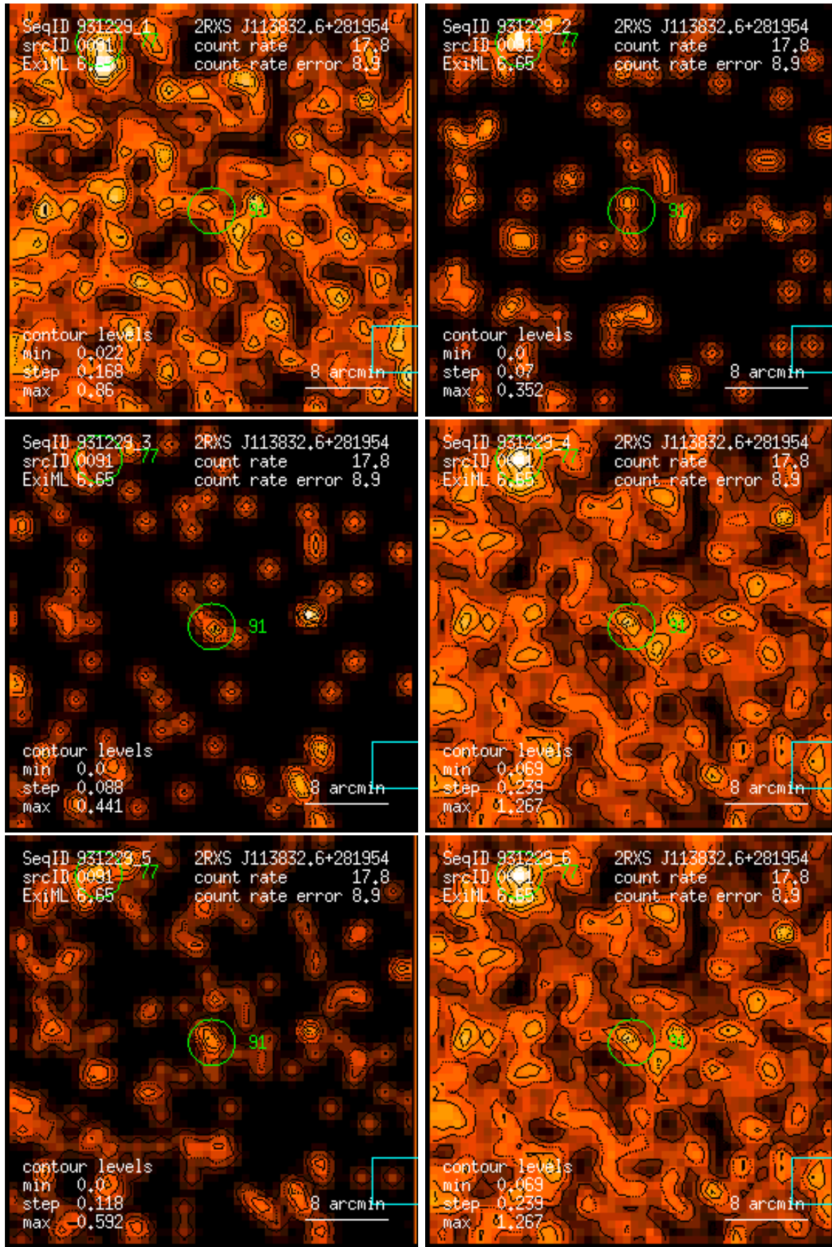
Figure 91: RASS 931229: detection 0091: band rate images, Gaussian filter: (1) PSPC channels 11 – 41, (2) 52 – 90, (3) 91 – 201, (4) 11 – 235, (5) 52 – 201, (6) 11 – 201. Broad band rates in counts/ks. Band rate contour levels in counts/ks/arcmin 2 .
