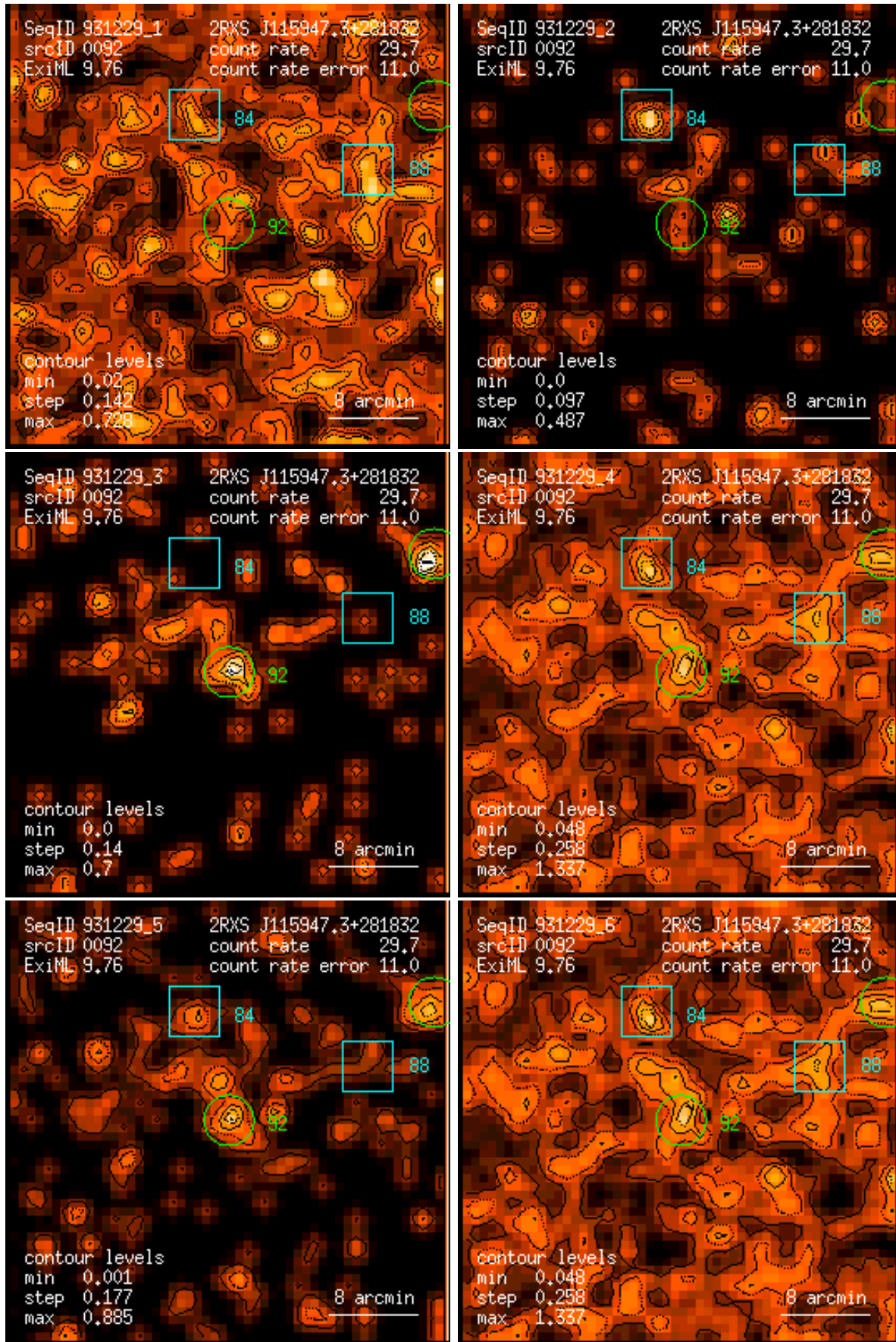
Figure 92: RASS 931229: detection 0092: band rate images, Gaussian filter: (1) PSPC channels 11 – 41, (2) 52 – 90, (3) 91 – 201, (4) 11 – 235, (5) 52 – 201, (6) 11 – 201. Broad band rates in counts/ks. Band rate contour levels in counts/ks/arcmin 2 .
